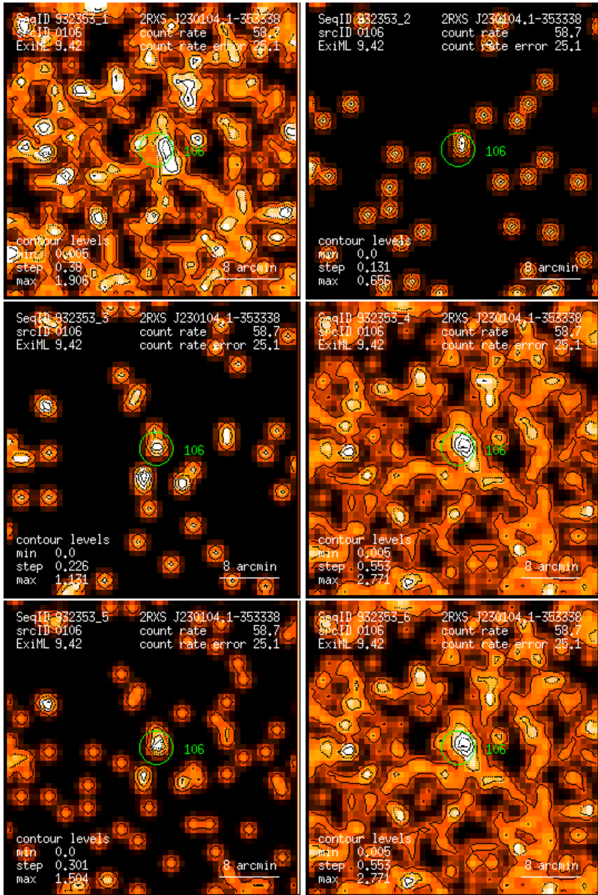
Figure 106: RASS 932353: detection 0106: band rate images, Gaussian filter: (1) PSPC channels 11 – 41, (2) 52 – 90, (3) 91 – 201, (4) 11 – 235, (5) 52 – 201, (6) 11 – 201. Broad band rates in counts/ks. Band rate contour levels in counts/ks/arcmin 2 .
