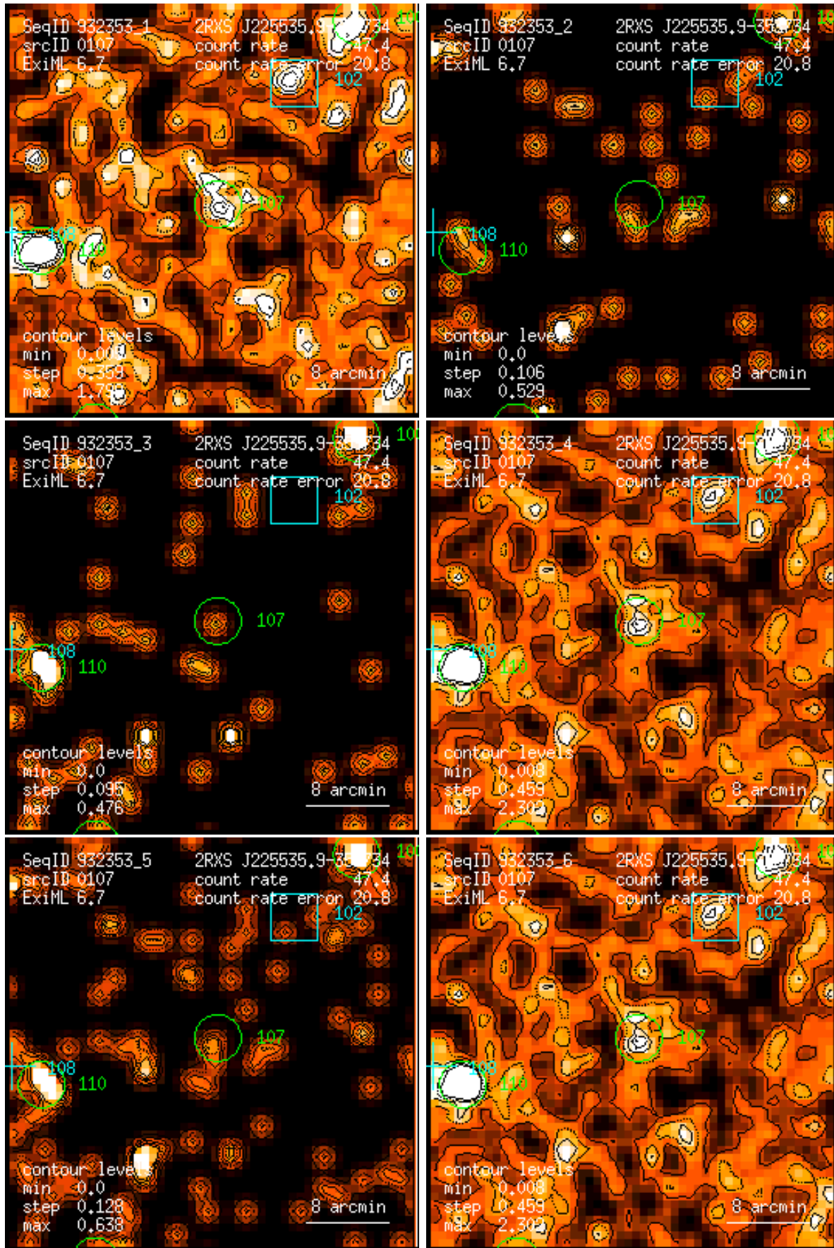
Figure 107: RASS 932353: detection 0107: band rate images, Gaussian filter: (1) PSPC channels 11 – 41, (2) 52 – 90, (3) 91 – 201, (4) 11 – 235, (5) 52 – 201, (6) 11 – 201. Broad band rates in counts/ks. Band rate contour levels in counts/ks/arcmin 2 .
