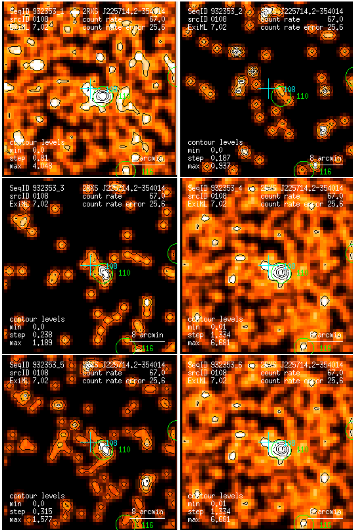
Figure 108: RASS 932353: detection 0108: band rate images, Gaussian filter: (1) PSPC channels 11 – 41, (2) 52 – 90, (3) 91 – 201, (4) 11 – 235, (5) 52 – 201, (6) 11 – 201. Broad band rates in counts/ks. Band rate contour levels in counts/ks/arcmin 2 .
