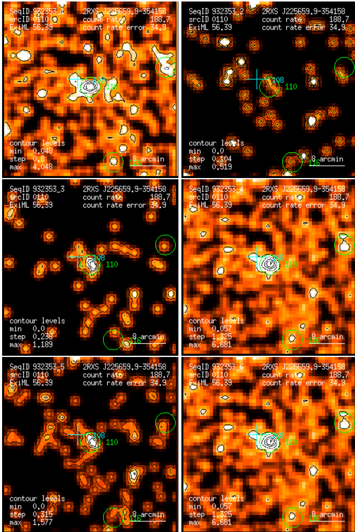
Figure 110: RASS 932353: detection 0110: band rate images, Gaussian filter: (1) PSPC channels 11 – 41, (2) 52 – 90, (3) 91 – 201, (4) 11 – 235, (5) 52 – 201, (6) 11 – 201. Broad band rates in counts/ks. Band rate contour levels in counts/ks/arcmin 2 .
