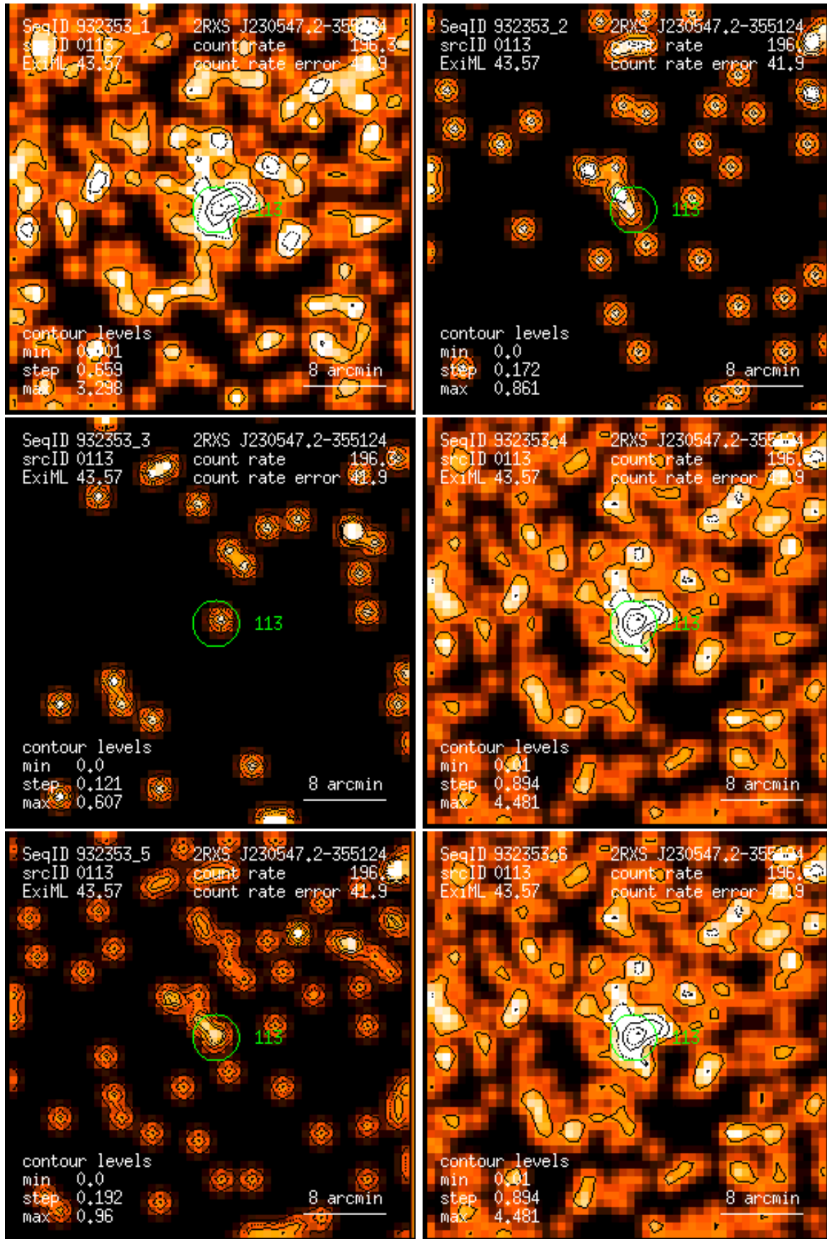
Figure 113: RASS 932353: detection 0113: band rate images, Gaussian filter: (1) PSPC channels 11 – 41, (2) 52 – 90, (3) 91 – 201, (4) 11 – 235, (5) 52 – 201, (6) 11 – 201. Broad band rates in counts/ks. Band rate contour levels in counts/ks/arcmin 2 .
