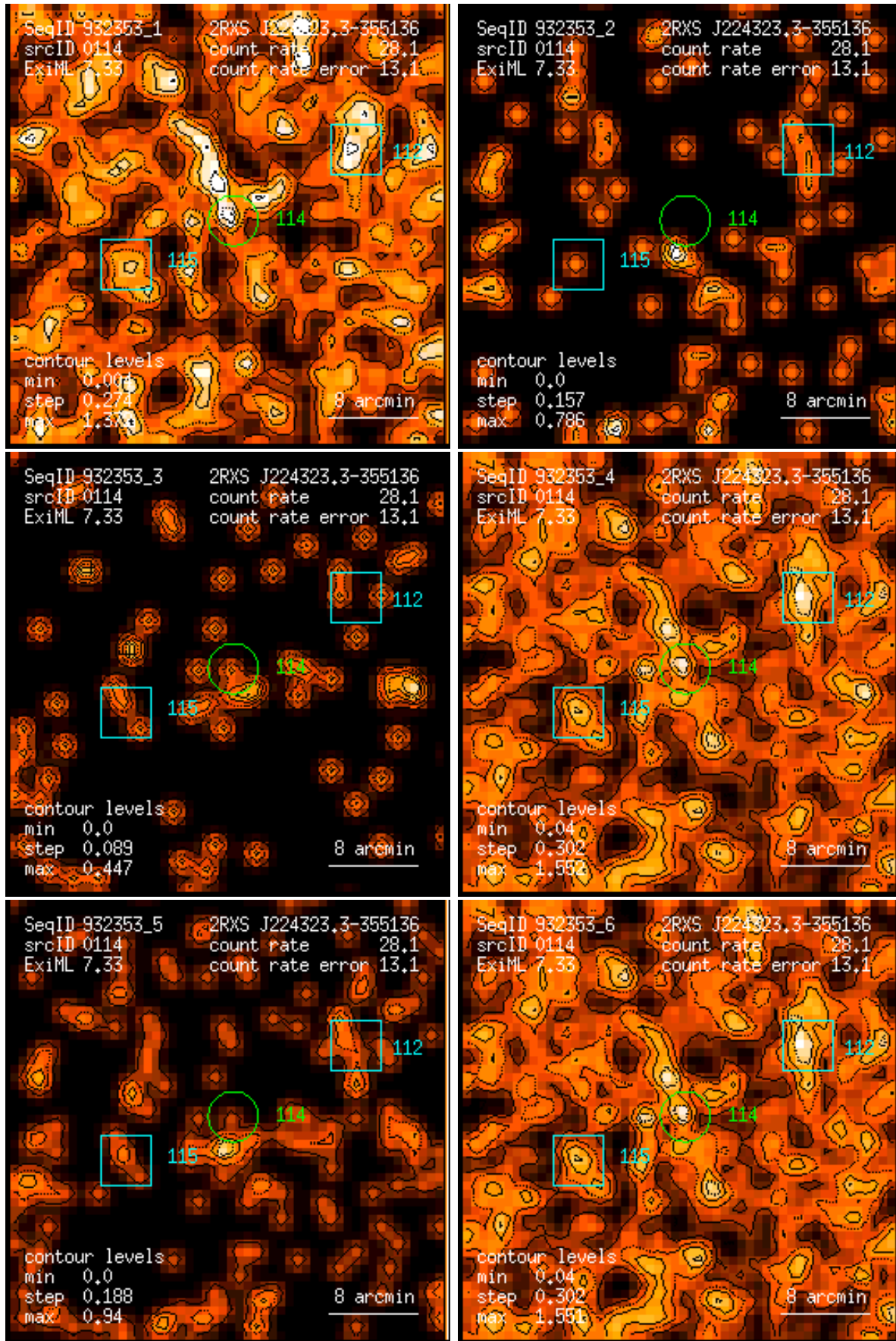
Figure 114: RASS 932353: detection 0114: band rate images, Gaussian filter: (1) PSPC channels 11 – 41, (2) 52 – 90, (3) 91 – 201, (4) 11 – 235, (5) 52 – 201, (6) 11 – 201. Broad band rates in counts/ks. Band rate contour levels in counts/ks/arcmin 2 .
