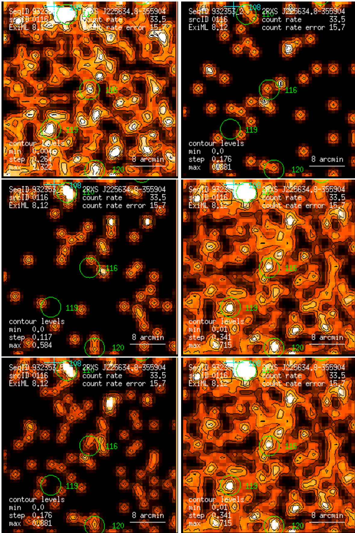
Figure 116: RASS 932353: detection 0116: band rate images, Gaussian filter: (1) PSPC channels 11 – 41, (2) 52 – 90, (3) 91 – 201, (4) 11 – 235, (5) 52 – 201, (6) 11 – 201. Broad band rates in counts/ks. Band rate contour levels in counts/ks/arcmin 2 .
