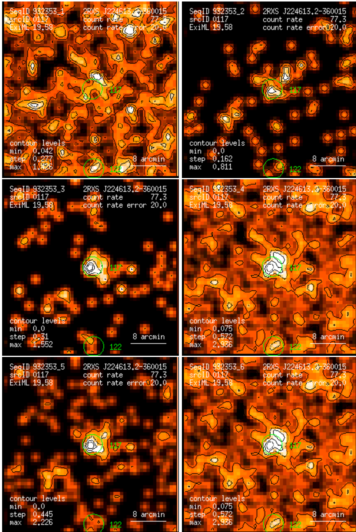
Figure 117: RASS 932353: detection 0117: band rate images, Gaussian filter: (1) PSPC channels 11 – 41, (2) 52 – 90, (3) 91 – 201, (4) 11 – 235, (5) 52 – 201, (6) 11 – 201. Broad band rates in counts/ks. Band rate contour levels in counts/ks/arcmin 2 .
