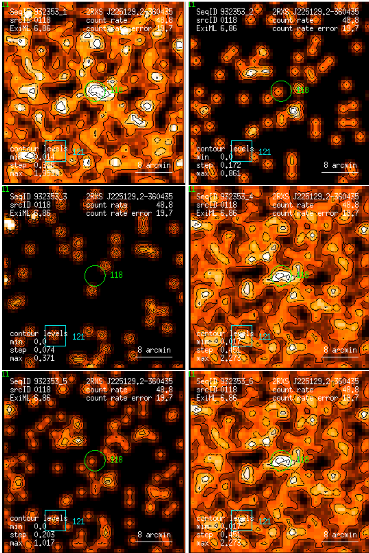
Figure 118: RASS 932353: detection 0118: band rate images, Gaussian filter: (1) PSPC channels 11 – 41, (2) 52 – 90, (3) 91 – 201, (4) 11 – 235, (5) 52 – 201, (6) 11 – 201. Broad band rates in counts/ks. Band rate contour levels in counts/ks/arcmin 2 .
