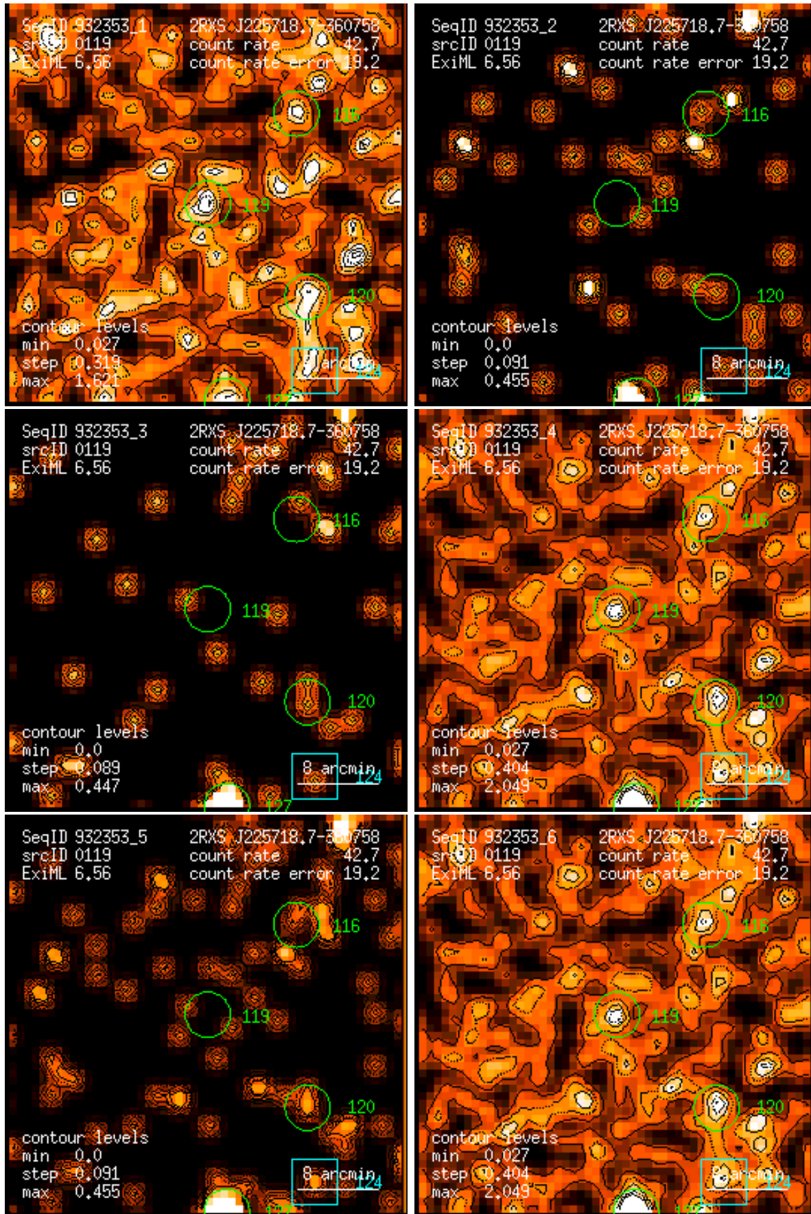
Figure 119: RASS 932353: detection 0119: band rate images, Gaussian filter: (1) PSPC channels 11 – 41, (2) 52 – 90, (3) 91 – 201, (4) 11 – 235, (5) 52 – 201, (6) 11 – 201. Broad band rates in counts/ks. Band rate contour levels in counts/ks/arcmin 2 .
