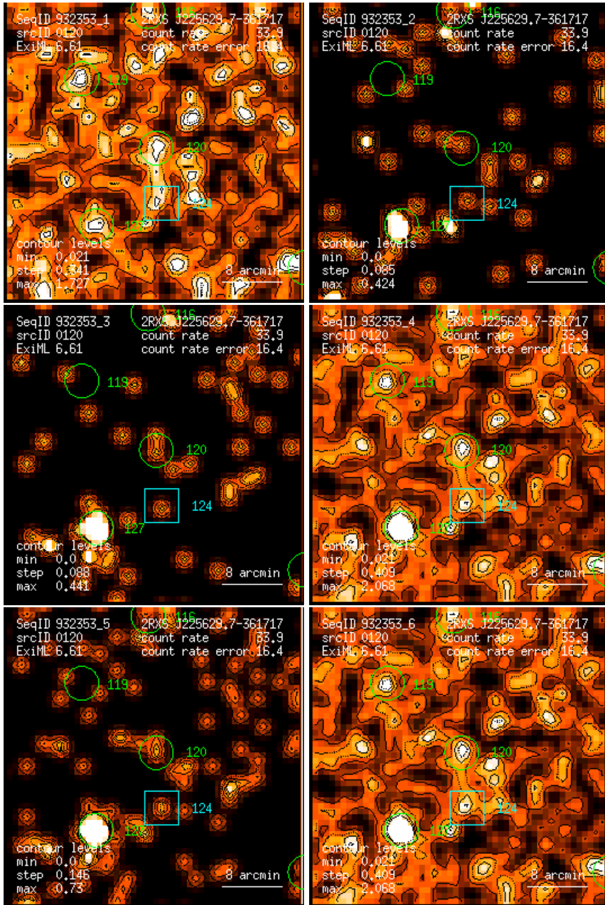
Figure 120: RASS 932353: detection 0120: band rate images, Gaussian filter: (1) PSPC channels 11 – 41, (2) 52 – 90, (3) 91 – 201, (4) 11 – 235, (5) 52 – 201, (6) 11 – 201. Broad band rates in counts/ks. Band rate contour levels in counts/ks/arcmin 2 .
