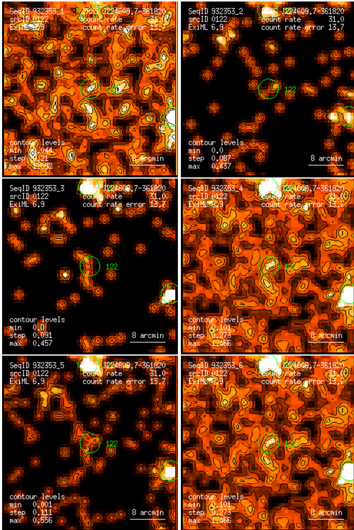
Figure 122: RASS 932353: detection 0122: band rate images, Gaussian filter: (1) PSPC channels 11 – 41, (2) 52 – 90, (3) 91 – 201, (4) 11 – 235, (5) 52 – 201, (6) 11 – 201. Broad band rates in counts/ks. Band rate contour levels in counts/ks/arcmin 2 .
