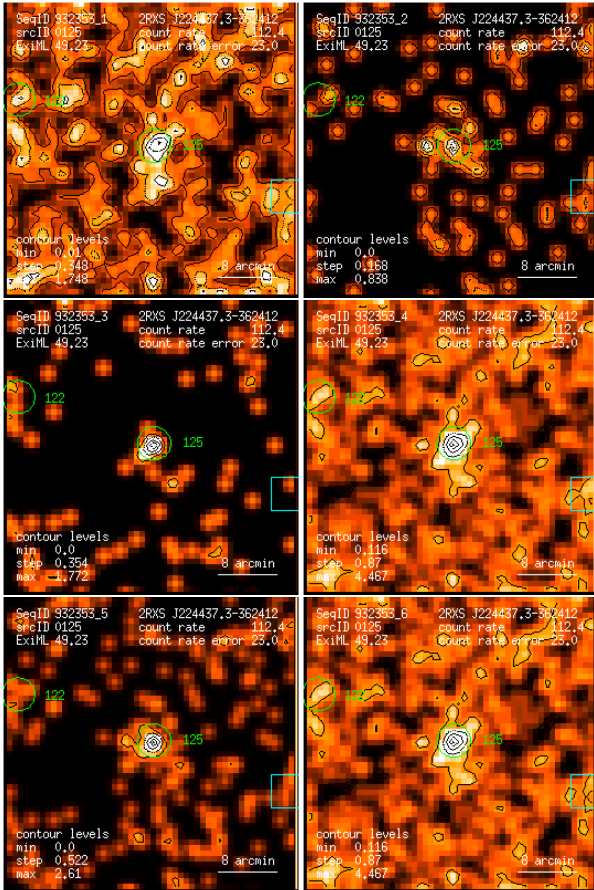
Figure 125: RASS 932353: detection 0125: band rate images, Gaussian filter: (1) PSPC channels 11 – 41, (2) 52 – 90, (3) 91 – 201, (4) 11 – 235, (5) 52 – 201, (6) 11 – 201. Broad band rates in counts/ks. Band rate contour levels in counts/ks/arcmin 2 .
