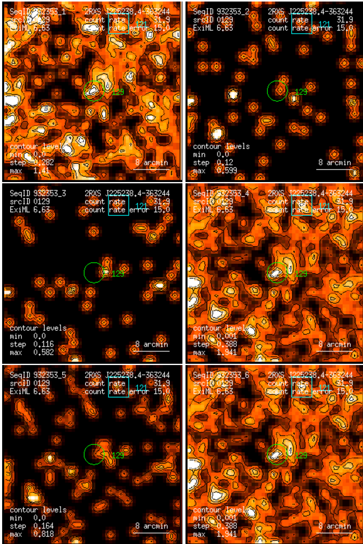
Figure 129: RASS 932353: detection 0129: band rate images, Gaussian filter: (1) PSPC channels 11 – 41, (2) 52 – 90, (3) 91 – 201, (4) 11 – 235, (5) 52 – 201, (6) 11 – 201. Broad band rates in counts/ks. Band rate contour levels in counts/ks/arcmin 2 .
