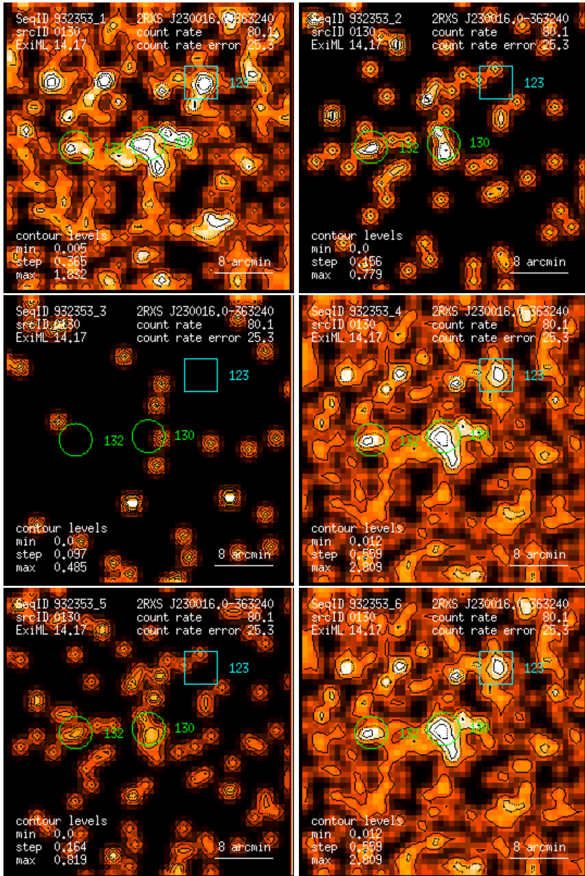
Figure 130: RASS 932353: detection 0130: band rate images, Gaussian filter: (1) PSPC channels 11 – 41, (2) 52 – 90, (3) 91 – 201, (4) 11 – 235, (5) 52 – 201, (6) 11 – 201. Broad band rates in counts/ks. Band rate contour levels in counts/ks/arcmin 2 .
