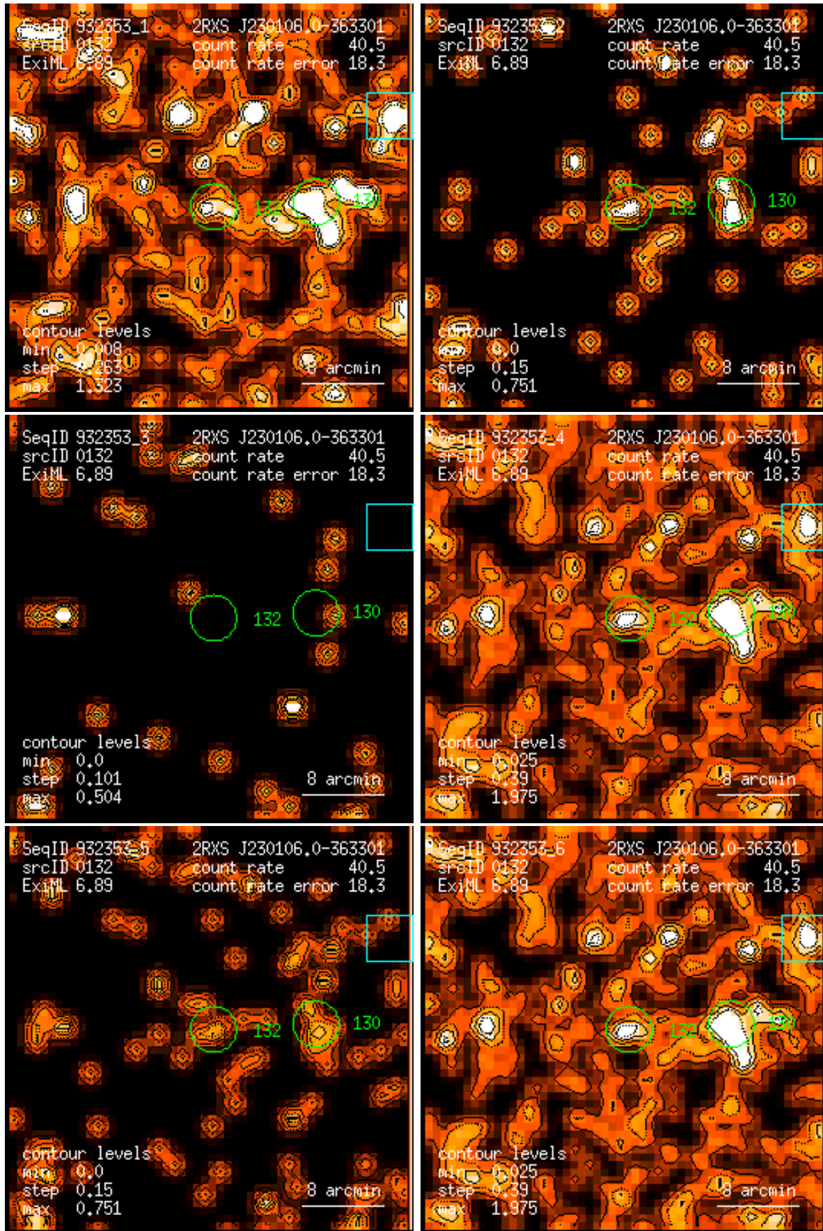
Figure 132: RASS 932353: detection 0132: band rate images, Gaussian filter: (1) PSPC channels 11 – 41, (2) 52 – 90, (3) 91 – 201, (4) 11 – 235, (5) 52 – 201, (6) 11 – 201. Broad band rates in counts/ks. Band rate contour levels in counts/ks/arcmin 2 .
