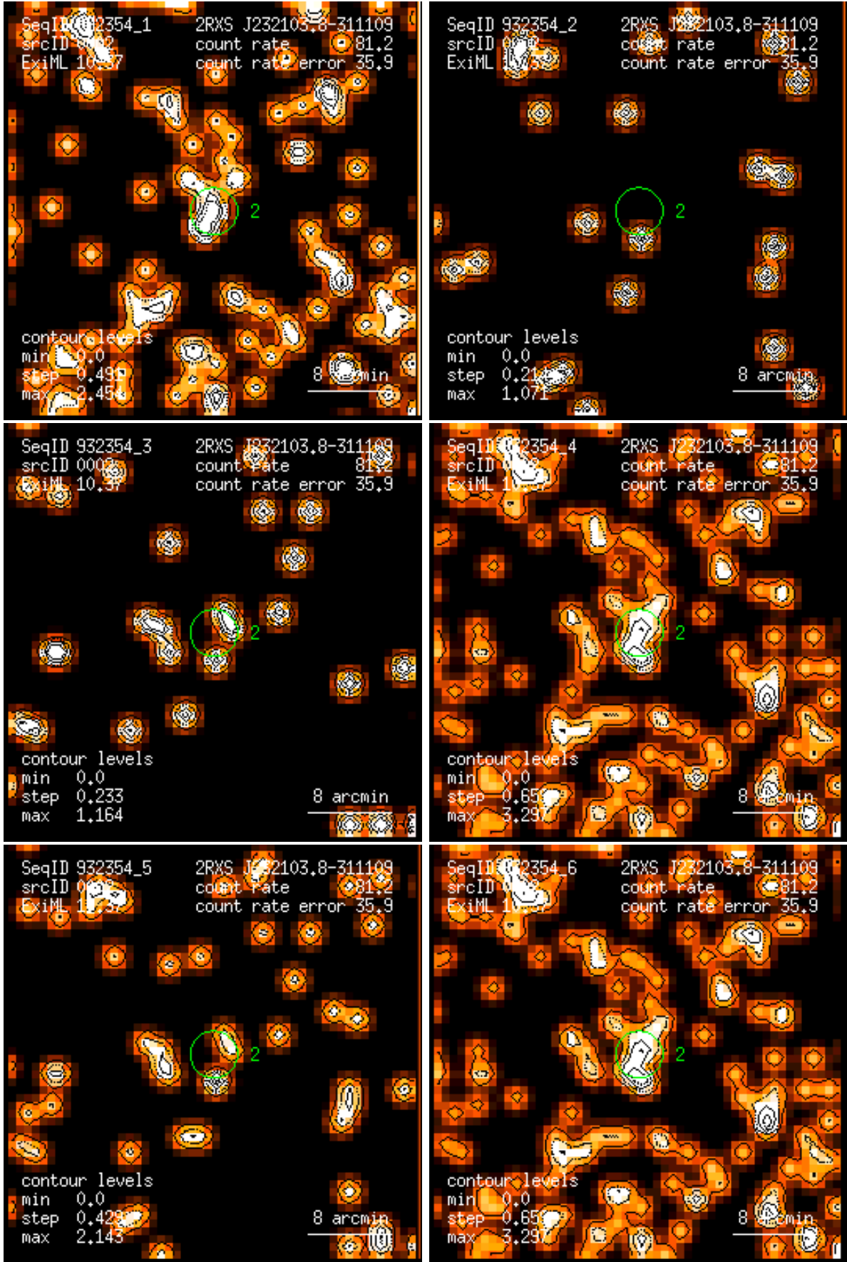
Figure 2: RASS 932354: detection 0002: band rate images, Gaussian filter: (1) PSPC channels 11 – 41, (2) 52 – 90, (3) 91 – 201, (4) 11 – 235, (5) 52 – 201, (6) 11 – 201. Broad band rates in counts/ks. Band rate contour levels in counts/ks/arcmin 2 .
