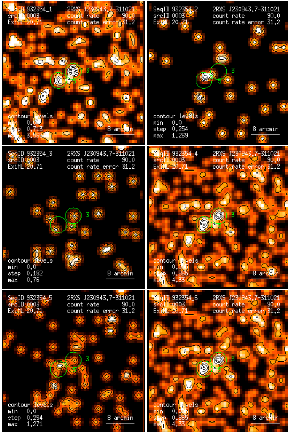
Figure 3: RASS 932354: detection 0003: band rate images, Gaussian filter: (1) PSPC channels 11 – 41, (2) 52 – 90, (3) 91 – 201, (4) 11 – 235, (5) 52 – 201, (6) 11 – 201. Broad band rates in counts/ks. Band rate contour levels in counts/ks/arcmin 2 .
