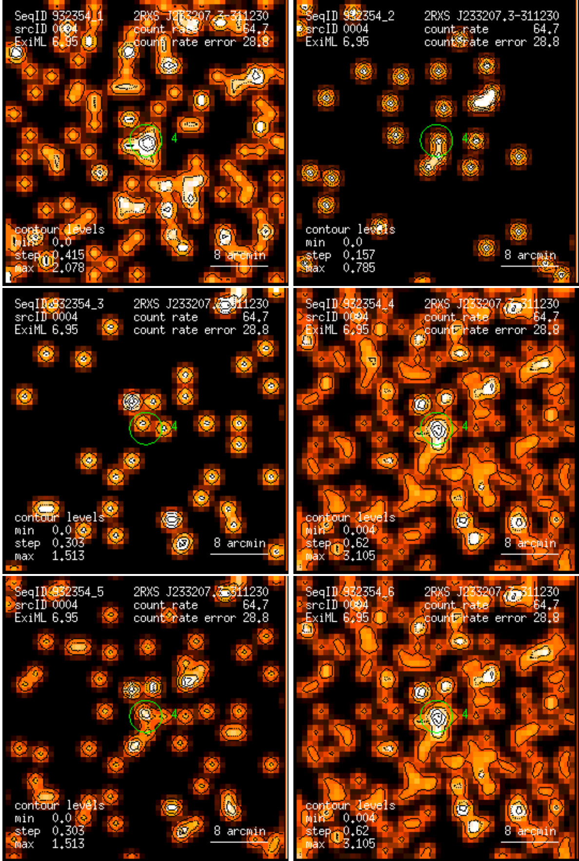
Figure 4: RASS 932354: detection 0004: band rate images, Gaussian filter: (1) PSPC channels 11 – 41, (2) 52 – 90, (3) 91 – 201, (4) 11 – 235, (5) 52 – 201, (6) 11 – 201. Broad band rates in counts/ks. Band rate contour levels in counts/ks/arcmin 2 .
