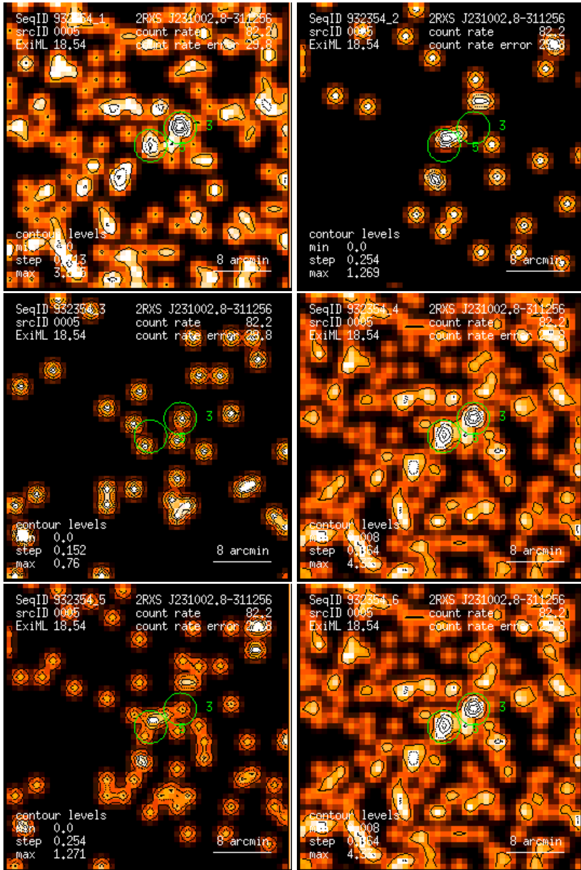
Figure 5: RASS 932354: detection 0005: band rate images, Gaussian filter: (1) PSPC channels 11 – 41, (2) 52 – 90, (3) 91 – 201, (4) 11 – 235, (5) 52 – 201, (6) 11 – 201. Broad band rates in counts/ks. Band rate contour levels in counts/ks/arcmin 2 .
