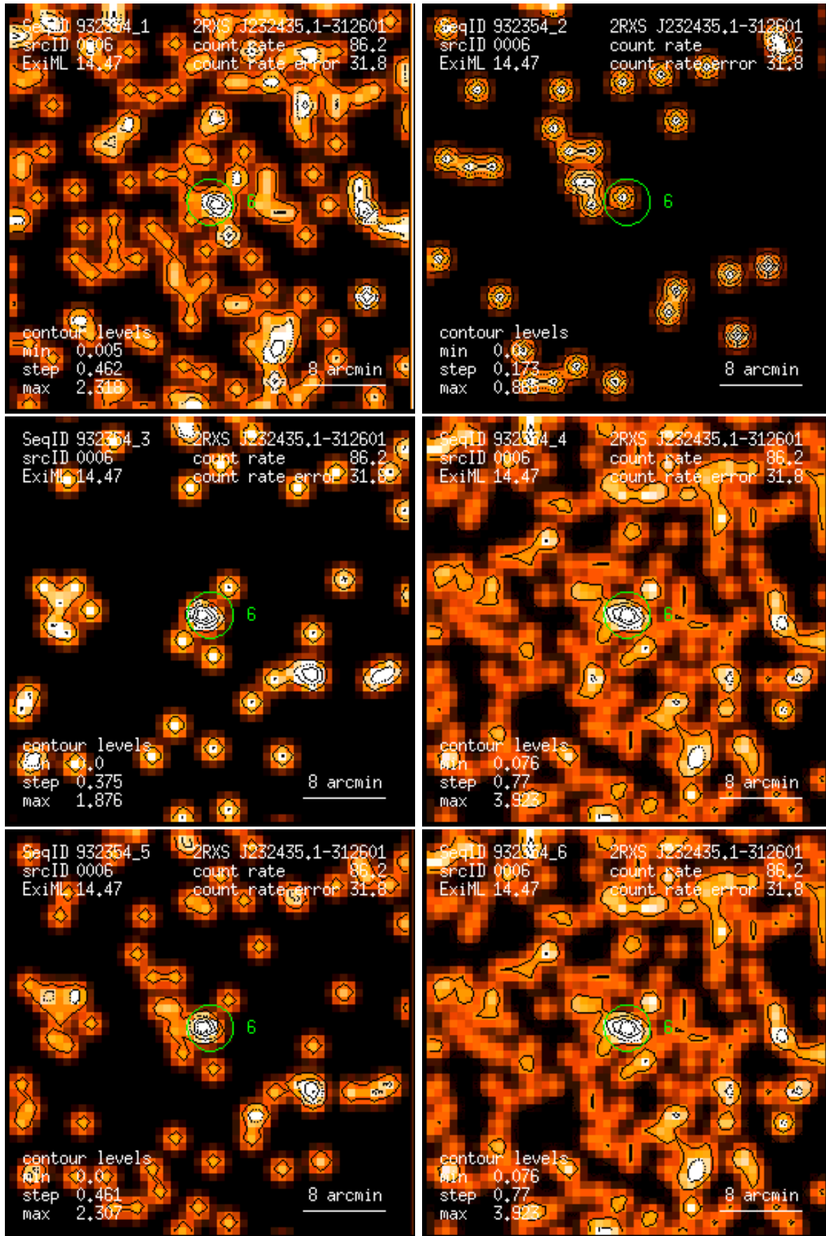
Figure 6: RASS 932354: detection 0006: band rate images, Gaussian filter: (1) PSPC channels 11 – 41, (2) 52 – 90, (3) 91 – 201, (4) 11 – 235, (5) 52 – 201, (6) 11 – 201. Broad band rates in counts/ks. Band rate contour levels in counts/ks/arcmin 2 .
