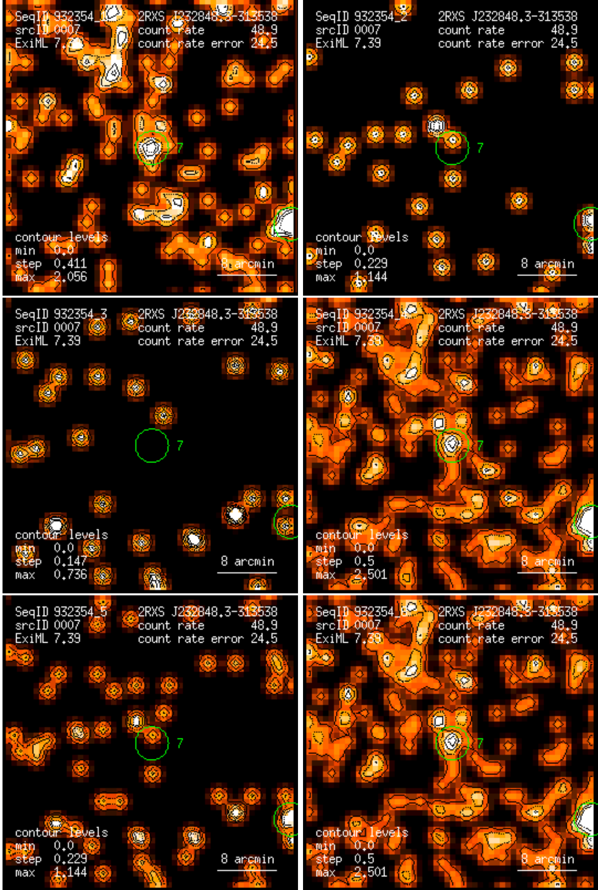
Figure 7: RASS 932354: detection 0007: band rate images, Gaussian filter: (1) PSPC channels 11 – 41, (2) 52 – 90, (3) 91 – 201, (4) 11 – 235, (5) 52 – 201, (6) 11 – 201. Broad band rates in counts/ks. Band rate contour levels in counts/ks/arcmin 2 .
