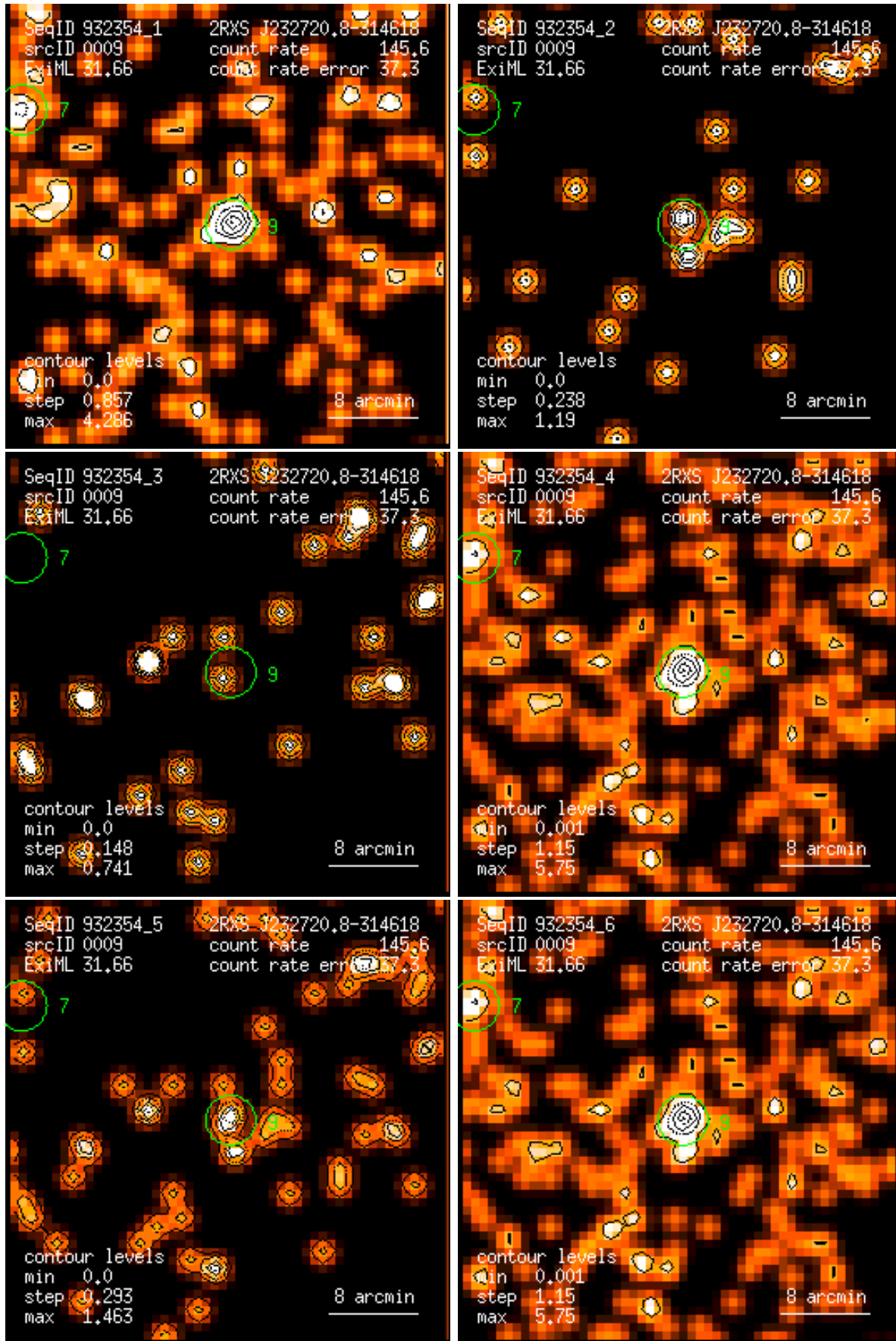
Figure 9: RASS 932354: detection 0009: band rate images, Gaussian filter: (1) PSPC channels 11 – 41, (2) 52 – 90, (3) 91 – 201, (4) 11 – 235, (5) 52 – 201, (6) 11 – 201. Broad band rates in counts/ks. Band rate contour levels in counts/ks/arcmin 2 .
