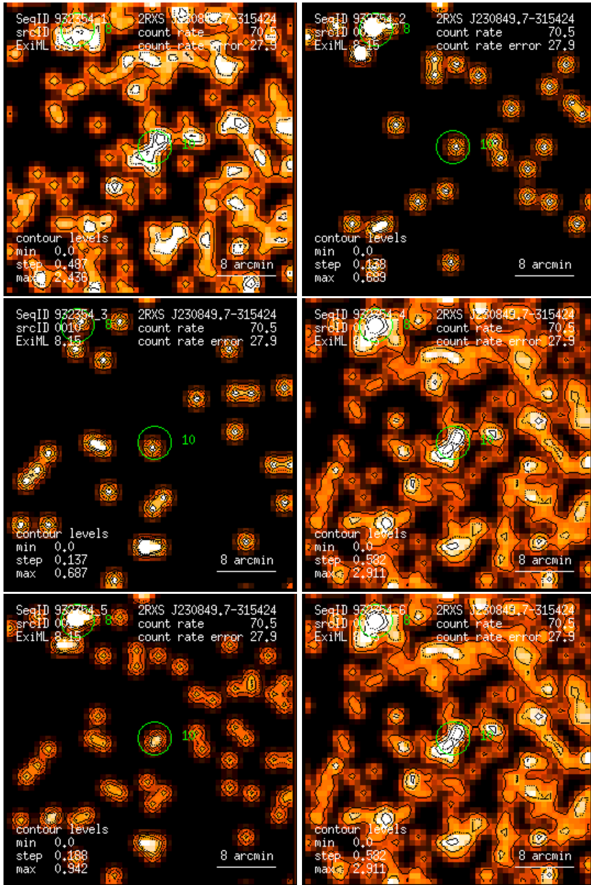
Figure 10: RASS 932354: detection 0010: band rate images, Gaussian filter: (1) PSPC channels 11 – 41, (2) 52 – 90, (3) 91 – 201, (4) 11 – 235, (5) 52 – 201, (6) 11 – 201. Broad band rates in counts/ks. Band rate contour levels in counts/ks/arcmin 2 .
