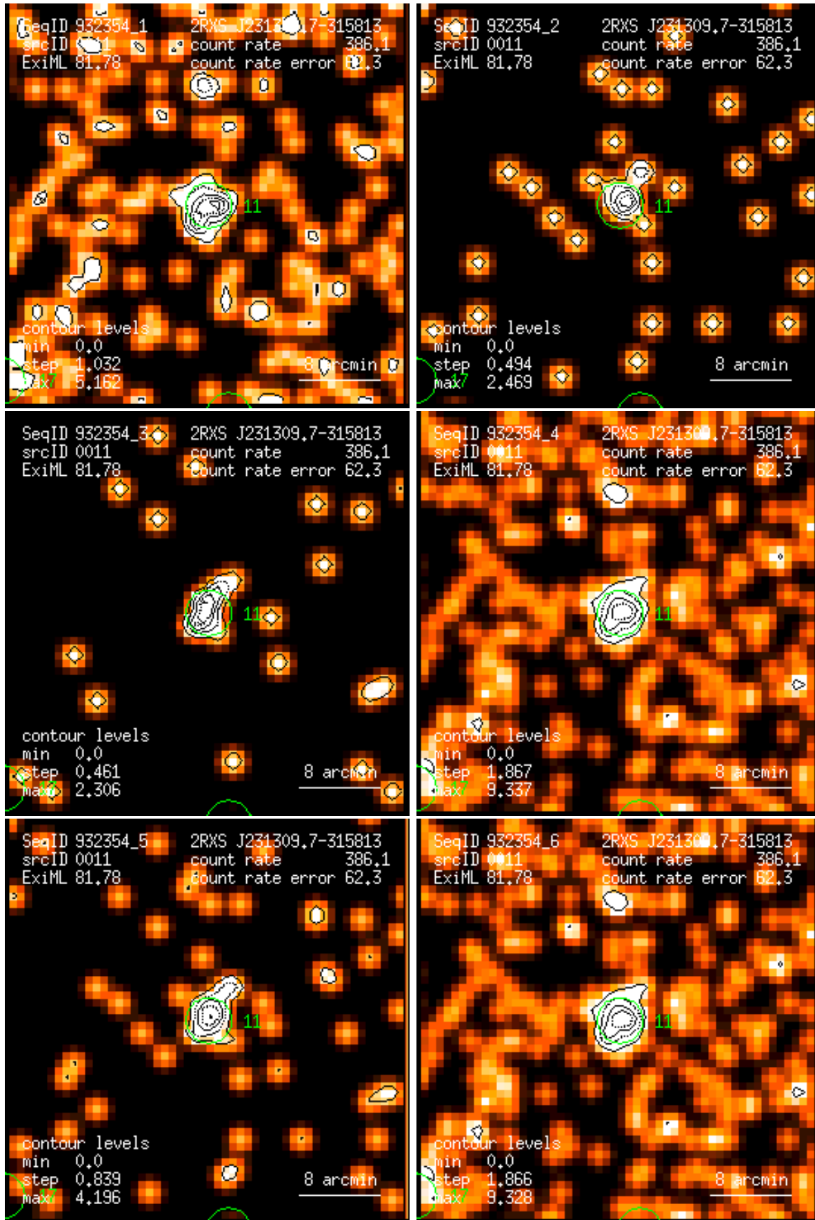
Figure 11: RASS 932354: detection 0011: band rate images, Gaussian filter: (1) PSPC channels 11 – 41, (2) 52 – 90, (3) 91 – 201, (4) 11 – 235, (5) 52 – 201, (6) 11 – 201. Broad band rates in counts/ks. Band rate contour levels in counts/ks/arcmin 2 .
