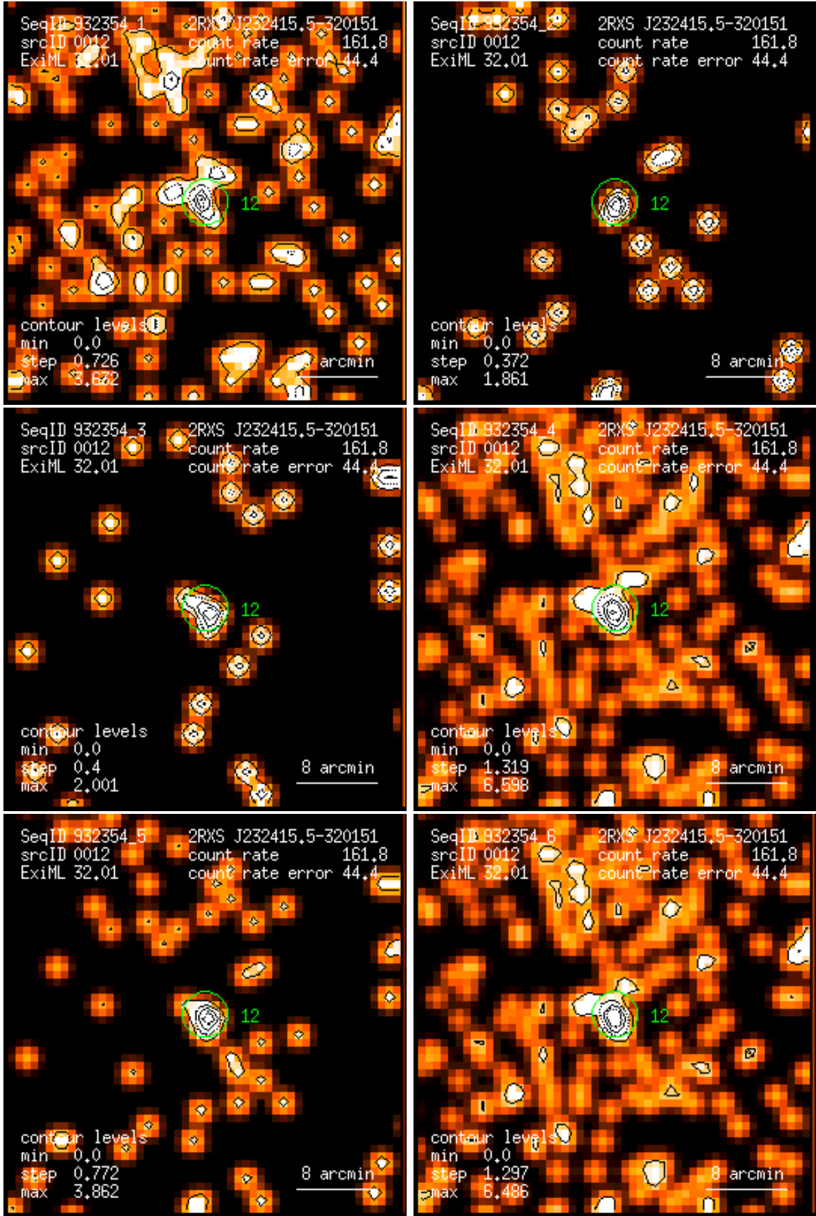
Figure 12: RASS 932354: detection 0012: band rate images, Gaussian filter: (1) PSPC channels 11 – 41, (2) 52 – 90, (3) 91 – 201, (4) 11 – 235, (5) 52 – 201, (6) 11 – 201. Broad band rates in counts/ks. Band rate contour levels in counts/ks/arcmin 2 .
