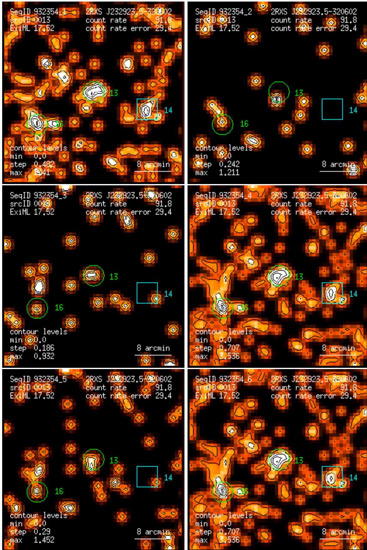
Figure 13: RASS 932354: detection 0013: band rate images, Gaussian filter: (1) PSPC channels 11 – 41, (2) 52 – 90, (3) 91 – 201, (4) 11 – 235, (5) 52 – 201, (6) 11 – 201. Broad band rates in counts/ks. Band rate contour levels in counts/ks/arcmin 2 .
