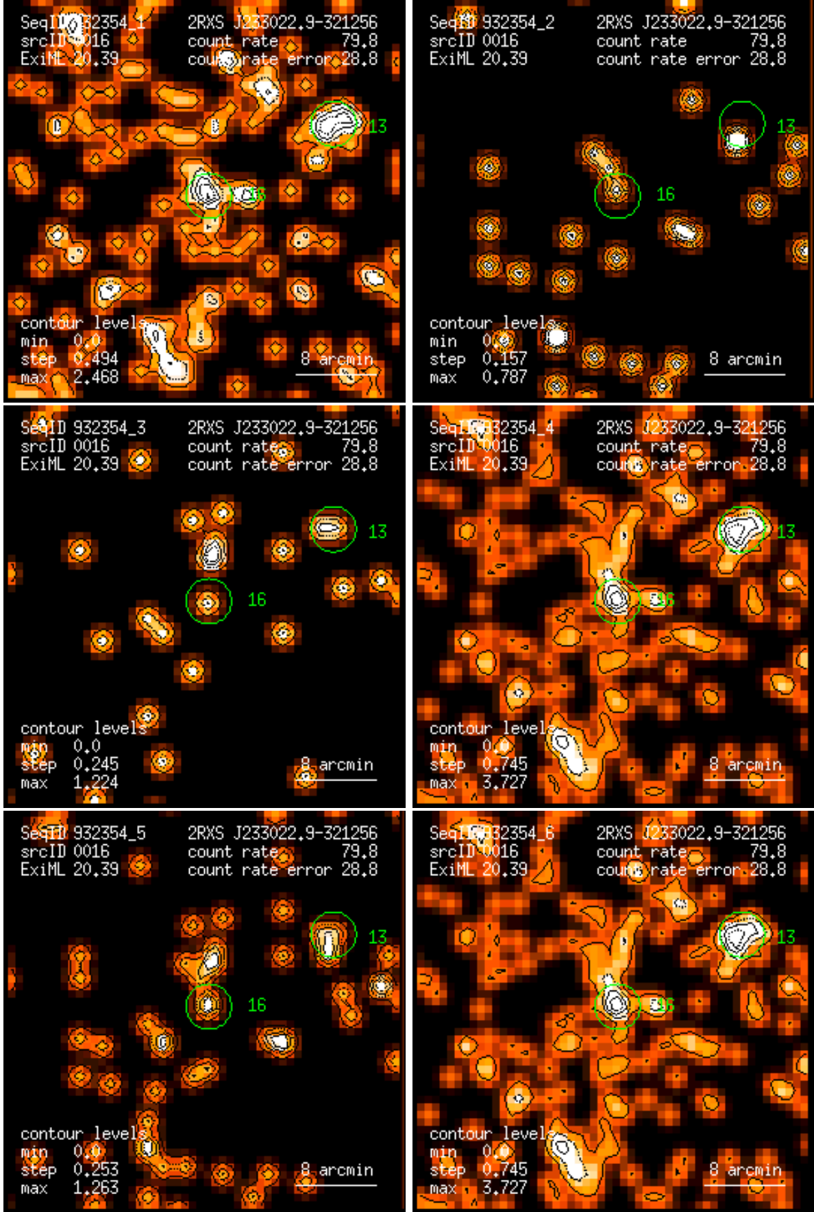
Figure 16: RASS 932354: detection 0016: band rate images, Gaussian filter: (1) PSPC channels 11 – 41, (2) 52 – 90, (3) 91 – 201, (4) 11 – 235, (5) 52 – 201, (6) 11 – 201. Broad band rates in counts/ks. Band rate contour levels in counts/ks/arcmin 2 .
