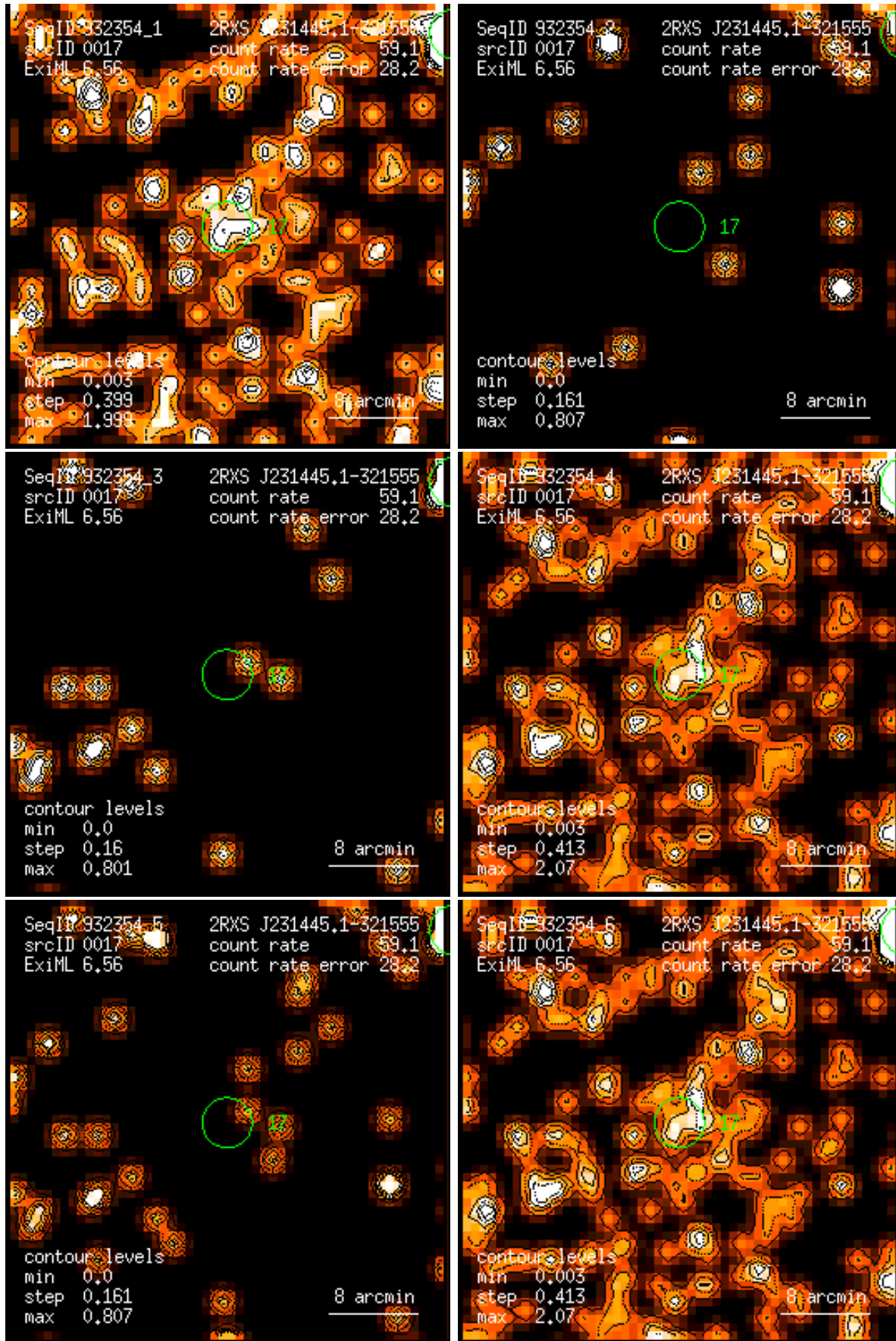
Figure 17: RASS 932354: detection 0017: band rate images, Gaussian filter: (1) PSPC channels 11 – 41, (2) 52 – 90, (3) 91 – 201, (4) 11 – 235, (5) 52 – 201, (6) 11 – 201. Broad band rates in counts/ks. Band rate contour levels in counts/ks/arcmin 2 .
