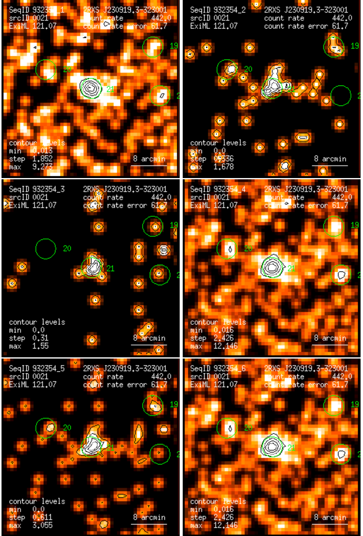
Figure 21: RASS 932354: detection 0021: band rate images, Gaussian filter: (1) PSPC channels 11 – 41, (2) 52 – 90, (3) 91 – 201, (4) 11 – 235, (5) 52 – 201, (6) 11 – 201. Broad band rates in counts/ks. Band rate contour levels in counts/ks/arcmin 2 .
