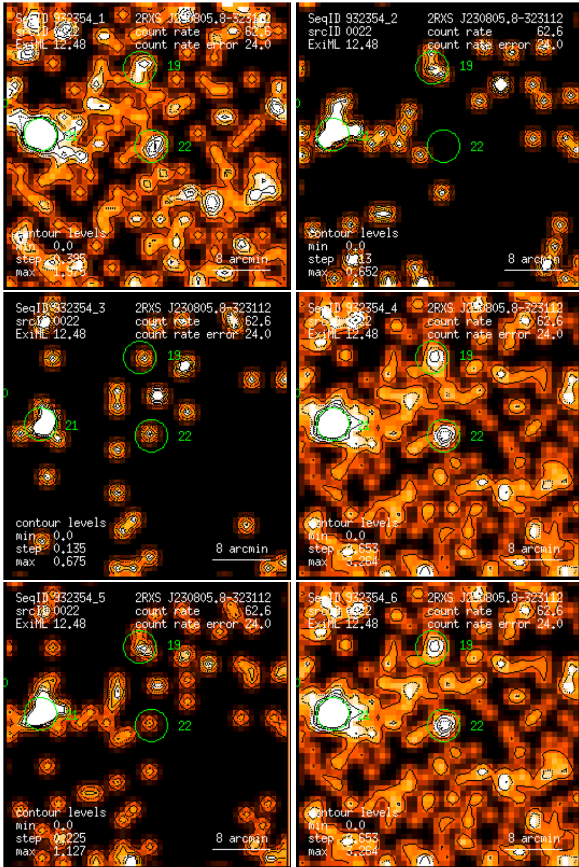
Figure 22: RASS 932354: detection 0022: band rate images, Gaussian filter: (1) PSPC channels 11 – 41, (2) 52 – 90, (3) 91 – 201, (4) 11 – 235, (5) 52 – 201, (6) 11 – 201. Broad band rates in counts/ks. Band rate contour levels in counts/ks/arcmin 2 .
