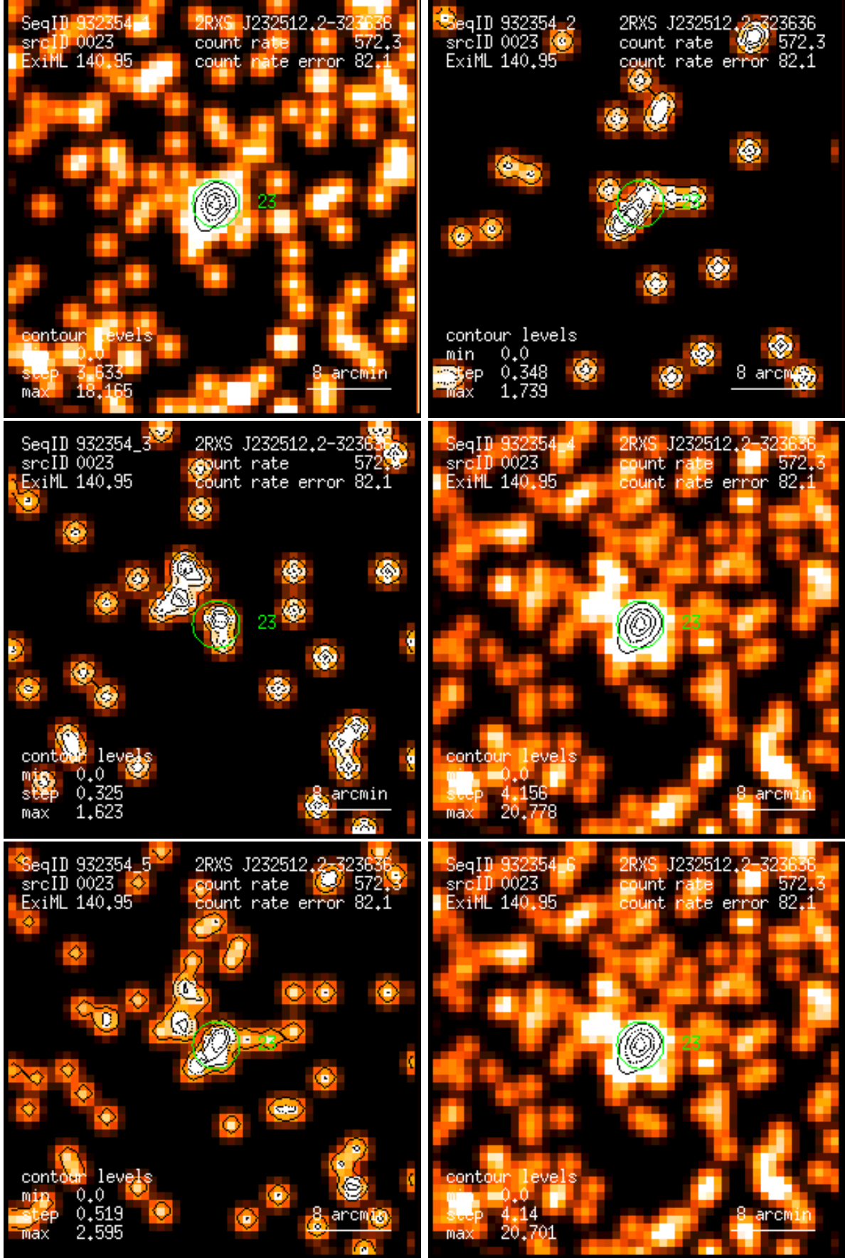
Figure 23: RASS 932354: detection 0023: band rate images, Gaussian filter: (1) PSPC channels 11 – 41, (2) 52 – 90, (3) 91 – 201, (4) 11 – 235, (5) 52 – 201, (6) 11 – 201. Broad band rates in counts/ks. Band rate contour levels in counts/ks/arcmin 2 .
