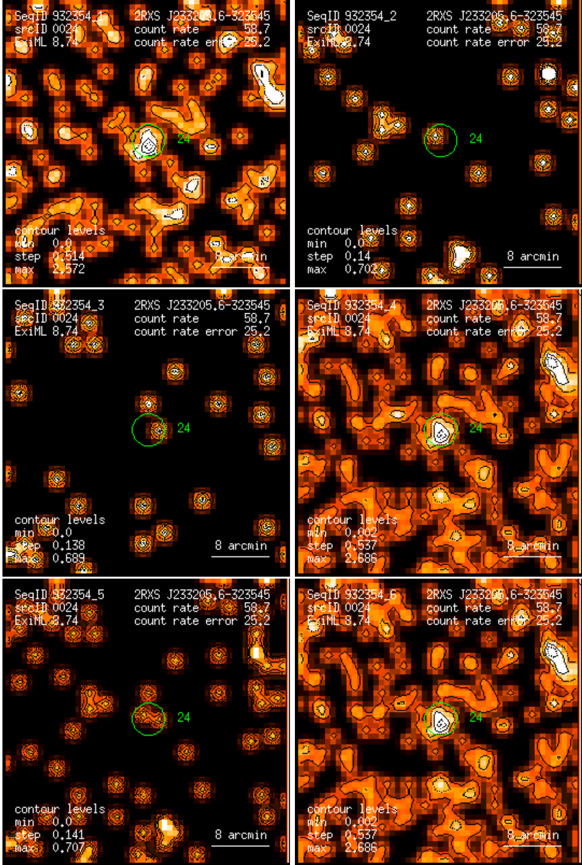
Figure 24: RASS 932354: detection 0024: band rate images, Gaussian filter: (1) PSPC channels 11 – 41, (2) 52 – 90, (3) 91 – 201, (4) 11 – 235, (5) 52 – 201, (6) 11 – 201. Broad band rates in counts/ks. Band rate contour levels in counts/ks/arcmin 2 .
