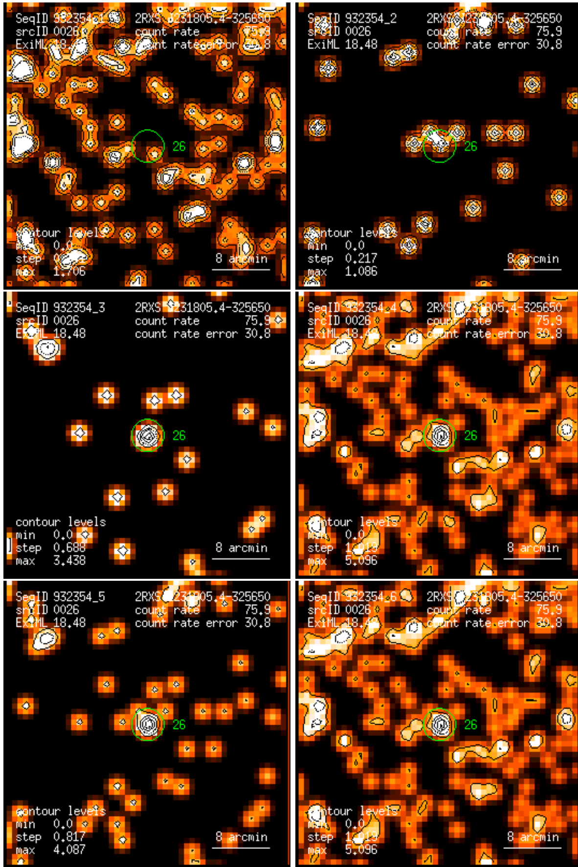
Figure 26: RASS 932354: detection 0026: band rate images, Gaussian filter: (1) PSPC channels 11 – 41, (2) 52 – 90, (3) 91 – 201, (4) 11 – 235, (5) 52 – 201, (6) 11 – 201. Broad band rates in counts/ks. Band rate contour levels in counts/ks/arcmin 2 .
