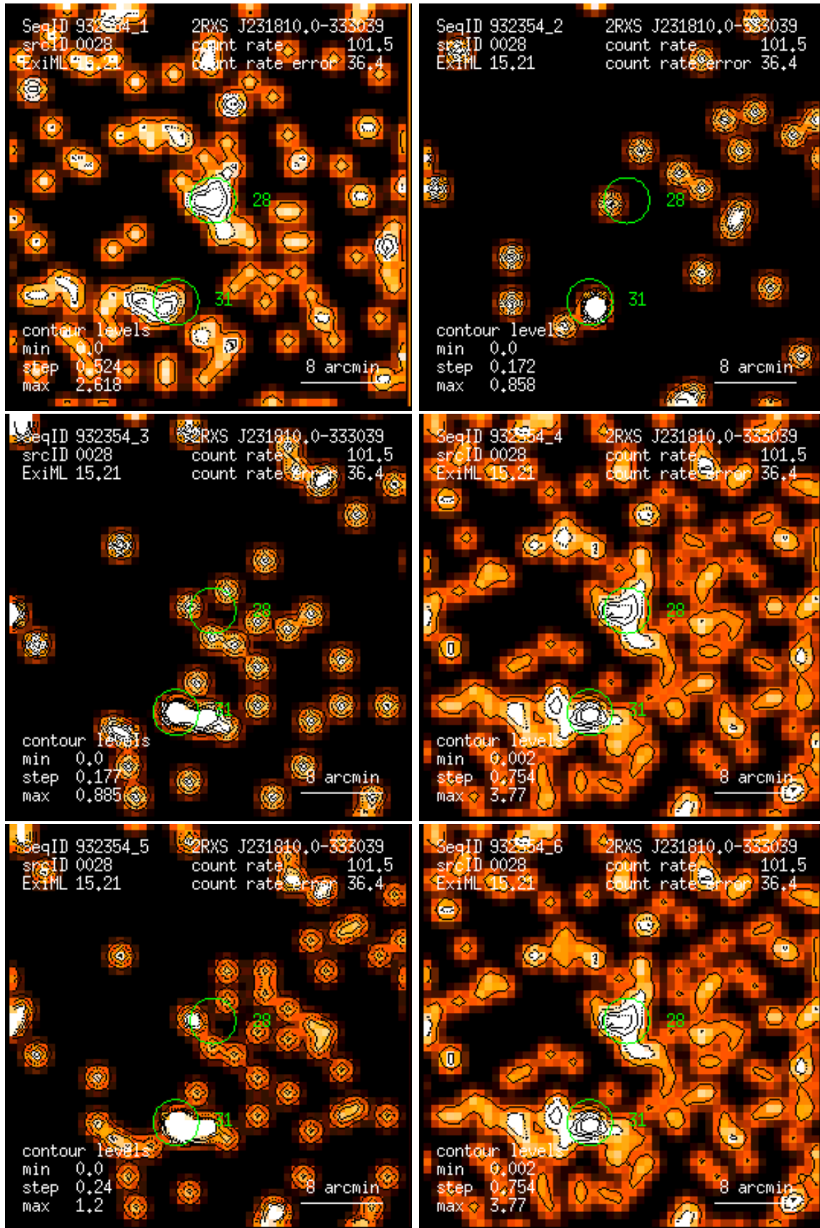
Figure 28: RASS 932354: detection 0028: band rate images, Gaussian filter: (1) PSPC channels 11 – 41, (2) 52 – 90, (3) 91 – 201, (4) 11 – 235, (5) 52 – 201, (6) 11 – 201. Broad band rates in counts/ks. Band rate contour levels in counts/ks/arcmin 2 .
