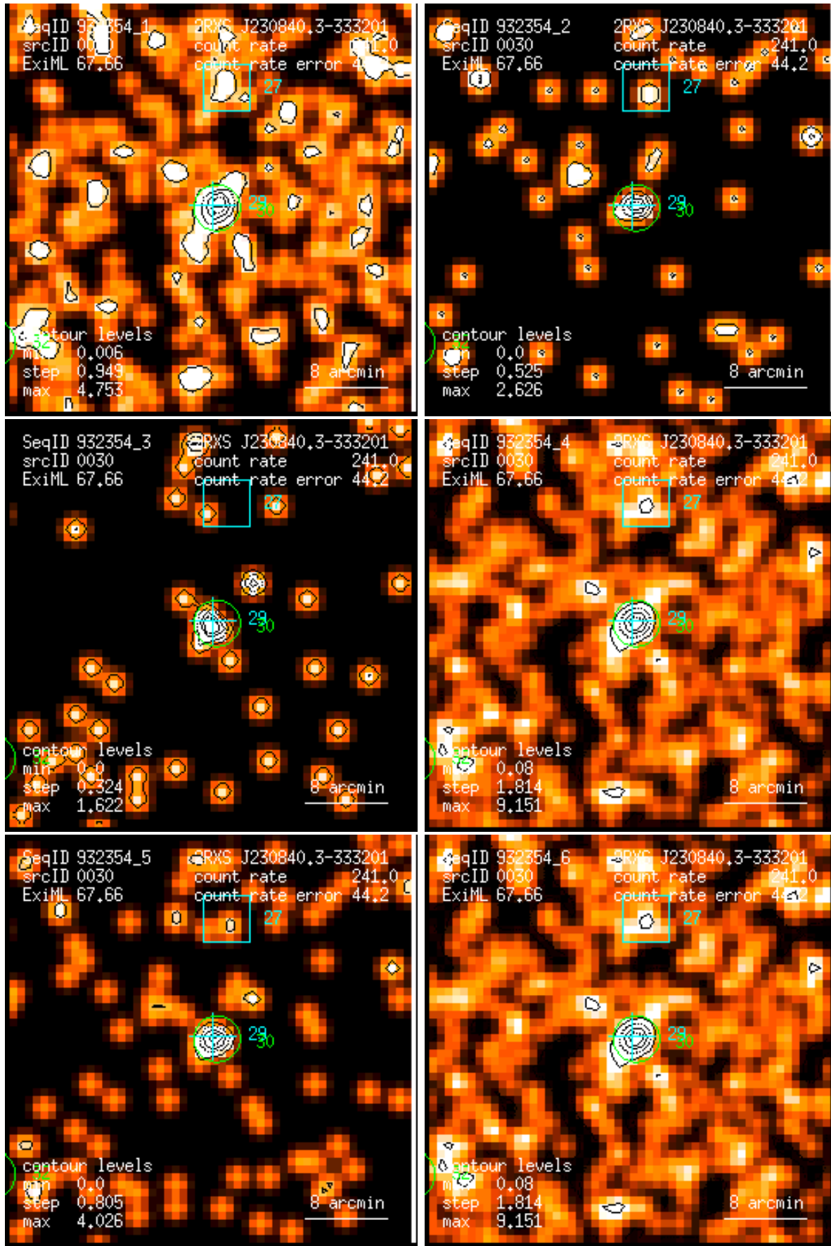
Figure 30: RASS 932354: detection 0030: band rate images, Gaussian filter: (1) PSPC channels 11 – 41, (2) 52 – 90, (3) 91 – 201, (4) 11 – 235, (5) 52 – 201, (6) 11 – 201. Broad band rates in counts/ks. Band rate contour levels in counts/ks/arcmin 2 .
