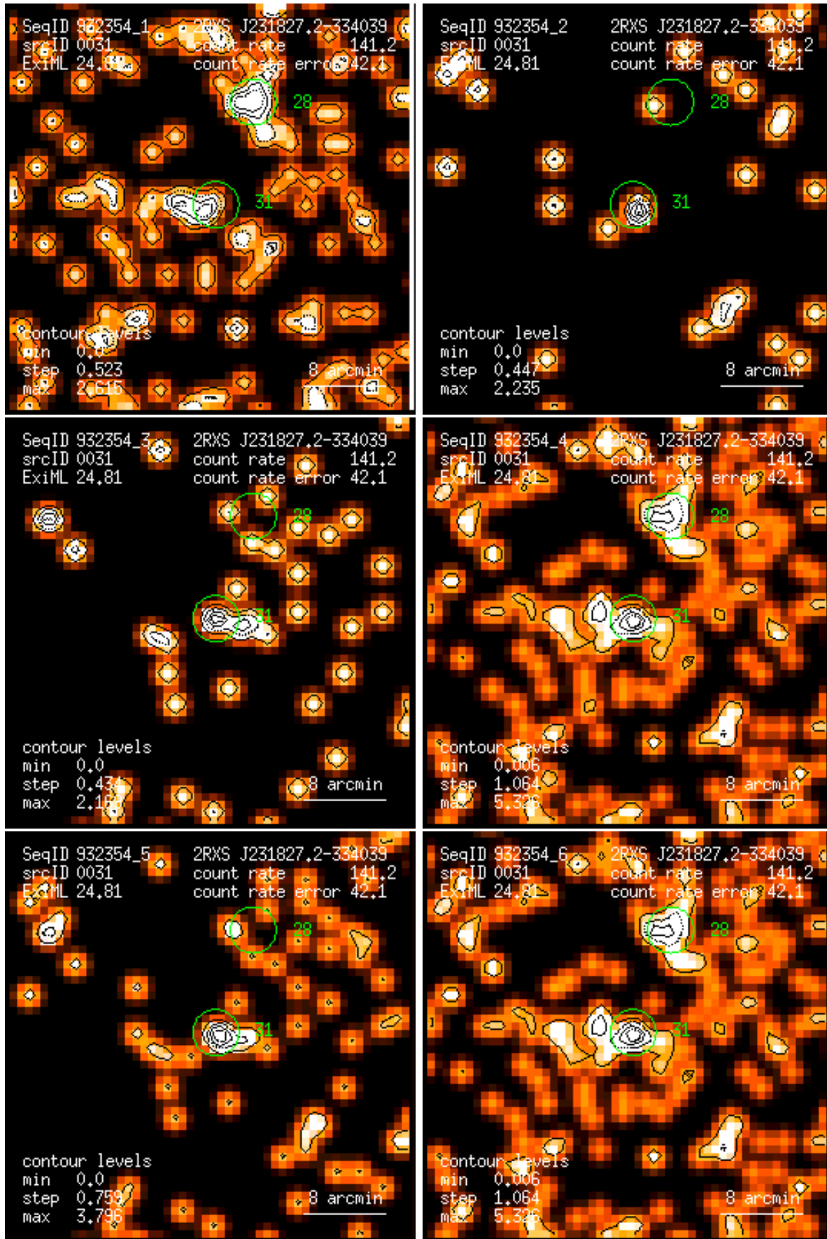
Figure 31: RASS 932354: detection 0031: band rate images, Gaussian filter: (1) PSPC channels 11 – 41, (2) 52 – 90, (3) 91 – 201, (4) 11 – 235, (5) 52 – 201, (6) 11 – 201. Broad band rates in counts/ks. Band rate contour levels in counts/ks/arcmin 2 .
