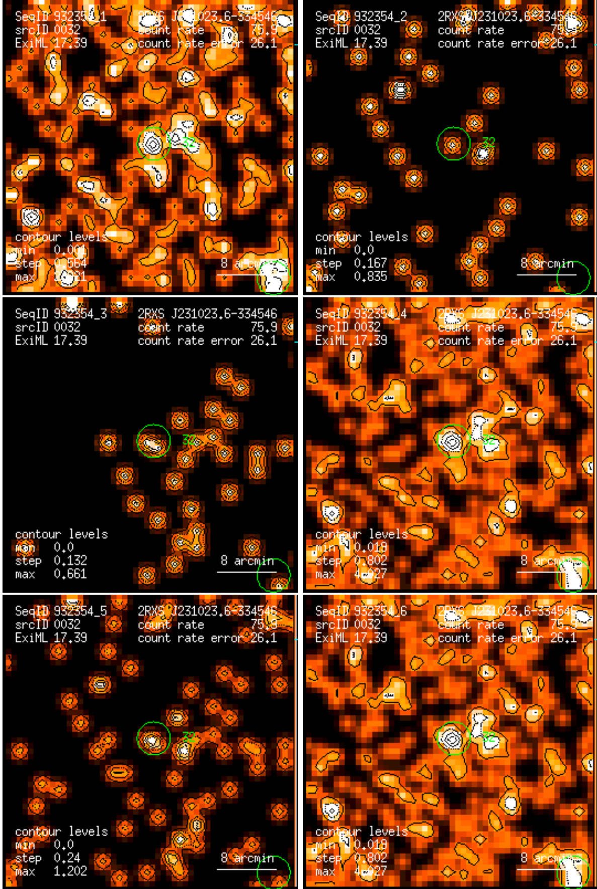
Figure 32: RASS 932354: detection 0032: band rate images, Gaussian filter: (1) PSPC channels 11 – 41, (2) 52 – 90, (3) 91 – 201, (4) 11 – 235, (5) 52 – 201, (6) 11 – 201. Broad band rates in counts/ks. Band rate contour levels in counts/ks/arcmin 2 .
