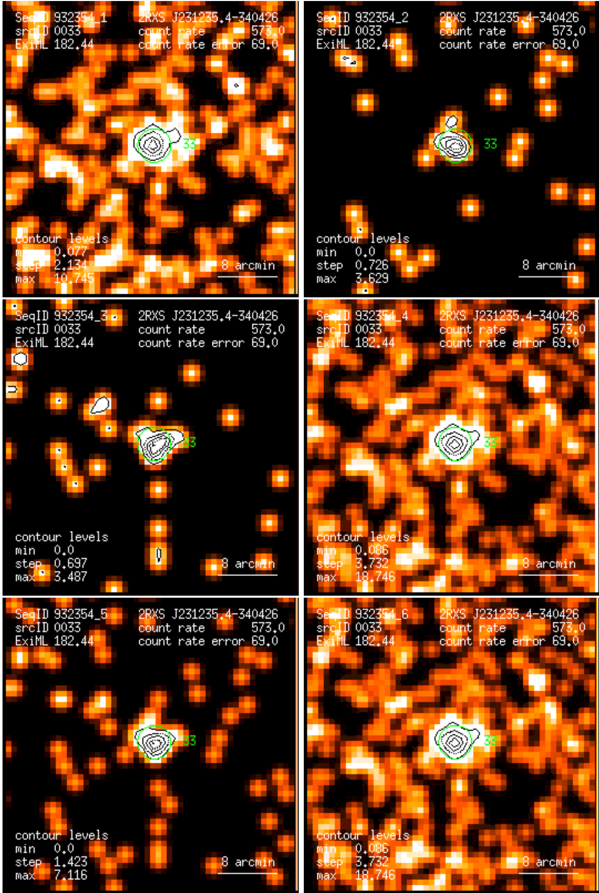
Figure 33: RASS 932354: detection 0033: band rate images, Gaussian filter: (1) PSPC channels 11 – 41, (2) 52 – 90, (3) 91 – 201, (4) 11 – 235, (5) 52 – 201, (6) 11 – 201. Broad band rates in counts/ks. Band rate contour levels in counts/ks/arcmin 2 .
