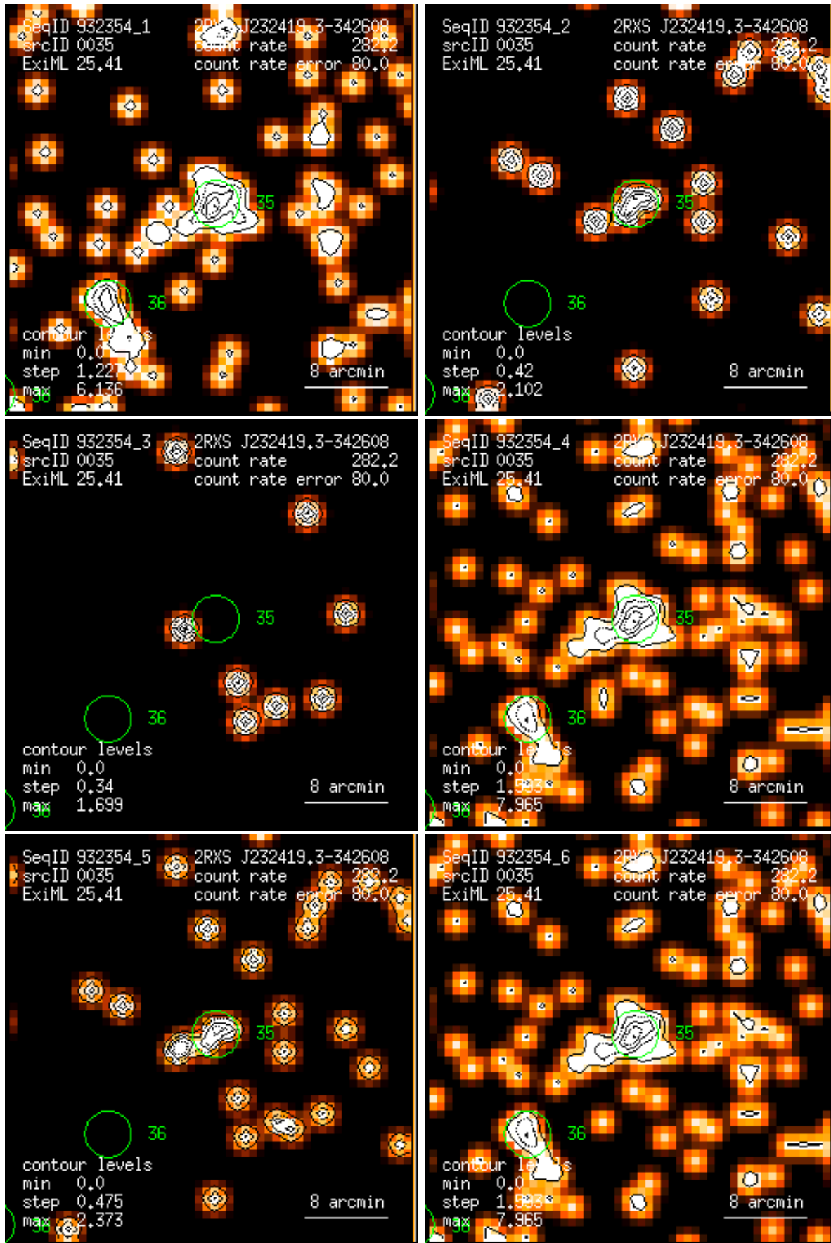
Figure 35: RASS 932354: detection 0035: band rate images, Gaussian filter: (1) PSPC channels 11 – 41, (2) 52 – 90, (3) 91 – 201, (4) 11 – 235, (5) 52 – 201, (6) 11 – 201. Broad band rates in counts/ks. Band rate contour levels in counts/ks/arcmin 2 .
