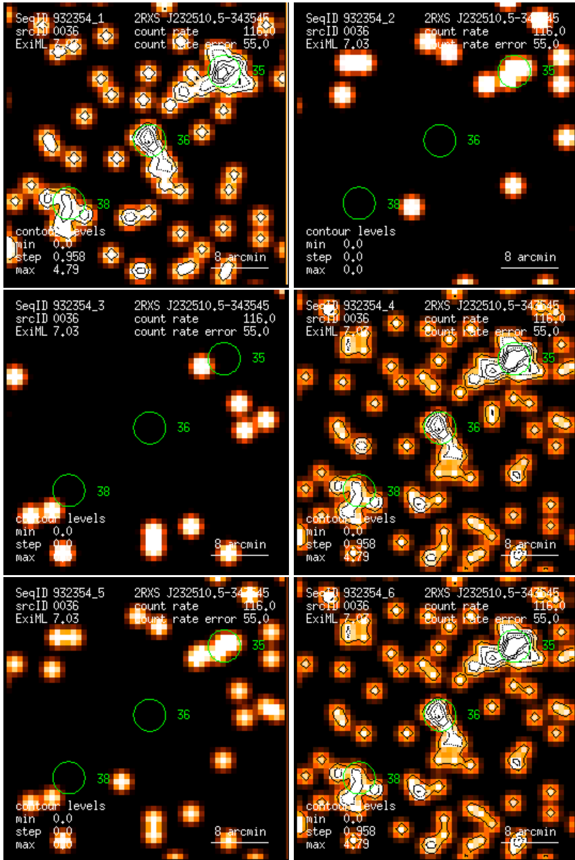
Figure 36: RASS 932354: detection 0036: band rate images, Gaussian filter: (1) PSPC channels 11 – 41, (2) 52 – 90, (3) 91 – 201, (4) 11 – 235, (5) 52 – 201, (6) 11 – 201. Broad band rates in counts/ks. Band rate contour levels in counts/ks/arcmin 2 .
