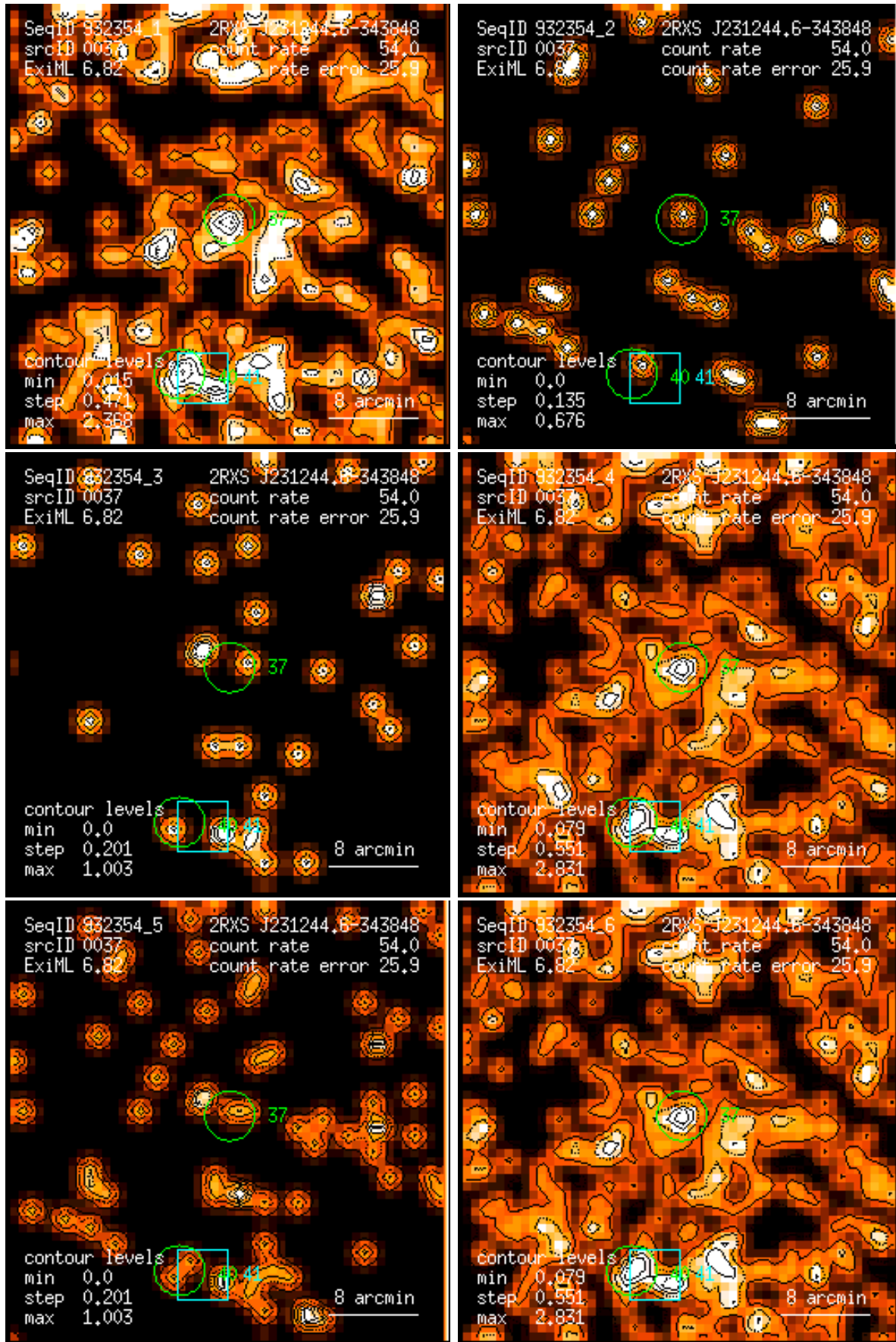
Figure 37: RASS 932354: detection 0037: band rate images, Gaussian filter: (1) PSPC channels 11 – 41, (2) 52 – 90, (3) 91 – 201, (4) 11 – 235, (5) 52 – 201, (6) 11 – 201. Broad band rates in counts/ks. Band rate contour levels in counts/ks/arcmin 2 .
