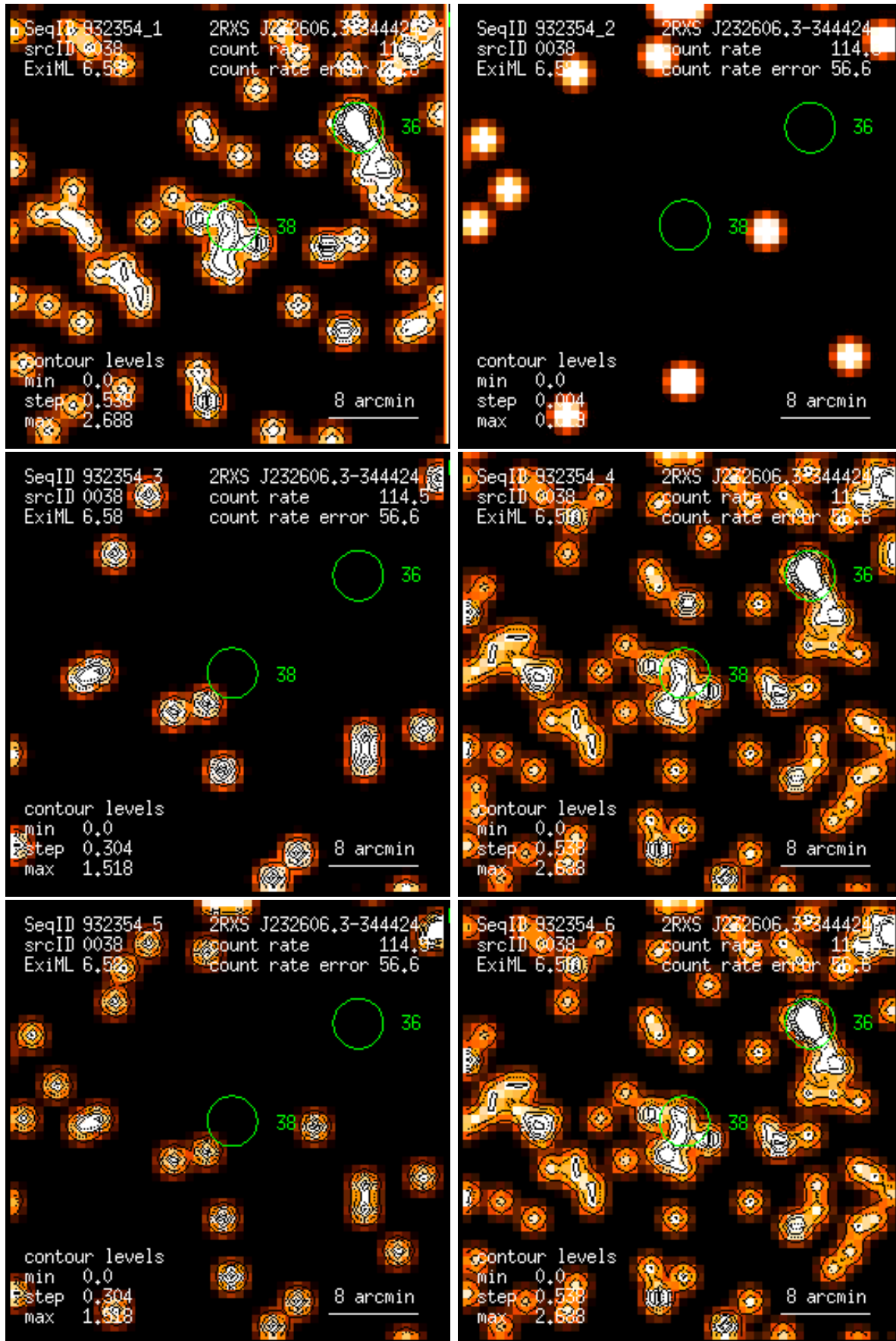
Figure 38: RASS 932354: detection 0038: band rate images, Gaussian filter: (1) PSPC channels 11 – 41, (2) 52 – 90, (3) 91 – 201, (4) 11 – 235, (5) 52 – 201, (6) 11 – 201. Broad band rates in counts/ks. Band rate contour levels in counts/ks/arcmin 2 .
