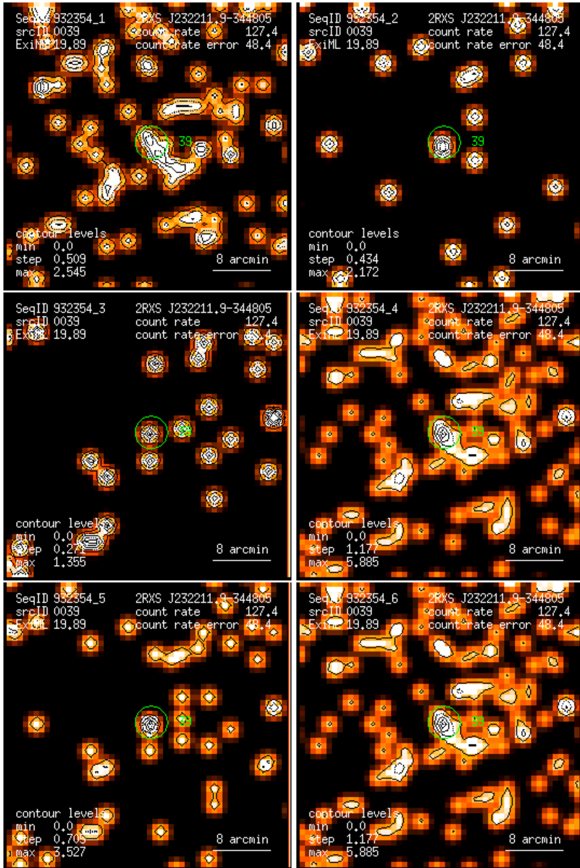
Figure 39: RASS 932354: detection 0039: band rate images, Gaussian filter: (1) PSPC channels 11 – 41, (2) 52 – 90, (3) 91 – 201, (4) 11 – 235, (5) 52 – 201, (6) 11 – 201. Broad band rates in counts/ks. Band rate contour levels in counts/ks/arcmin 2 .
