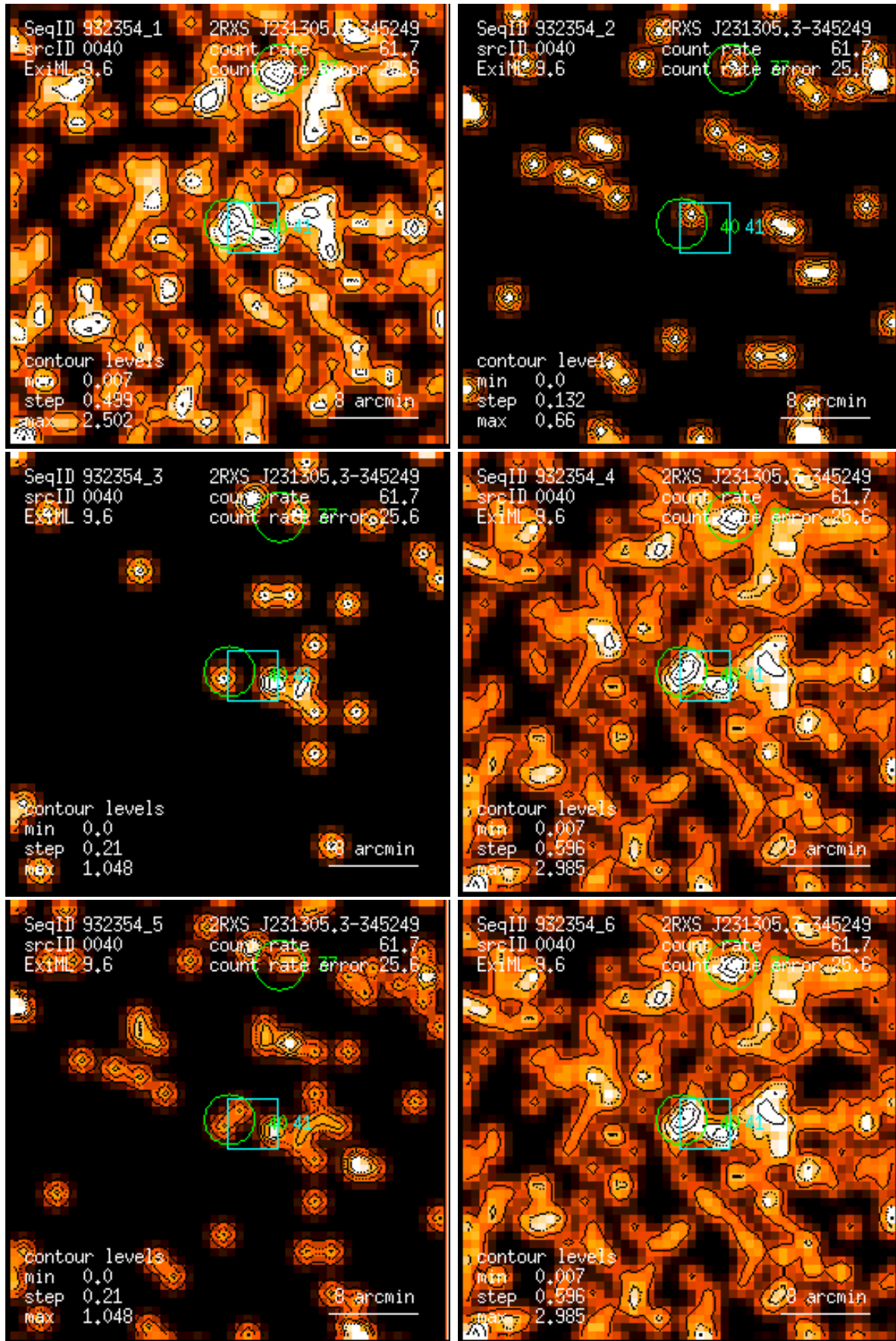
Figure 40: RASS 932354: detection 0040: band rate images, Gaussian filter: (1) PSPC channels 11 – 41, (2) 52 – 90, (3) 91 – 201, (4) 11 – 235, (5) 52 – 201, (6) 11 – 201. Broad band rates in counts/ks. Band rate contour levels in counts/ks/arcmin 2 .
