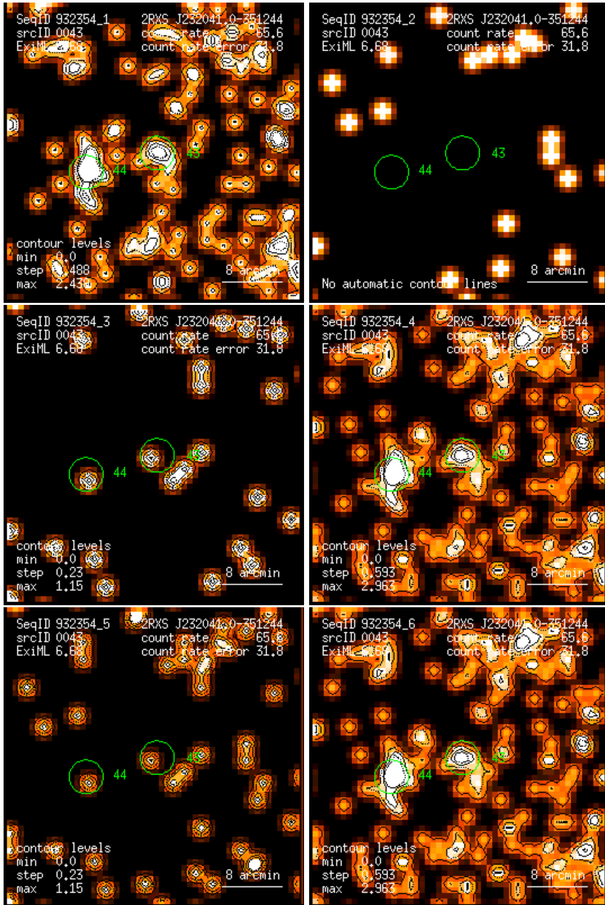
Figure 43: RASS 932354: detection 0043: band rate images, Gaussian filter: (1) PSPC channels 11 – 41, (2) 52 – 90, (3) 91 – 201, (4) 11 – 235, (5) 52 – 201, (6) 11 – 201. Broad band rates in counts/ks. Band rate contour levels in counts/ks/arcmin 2 .
