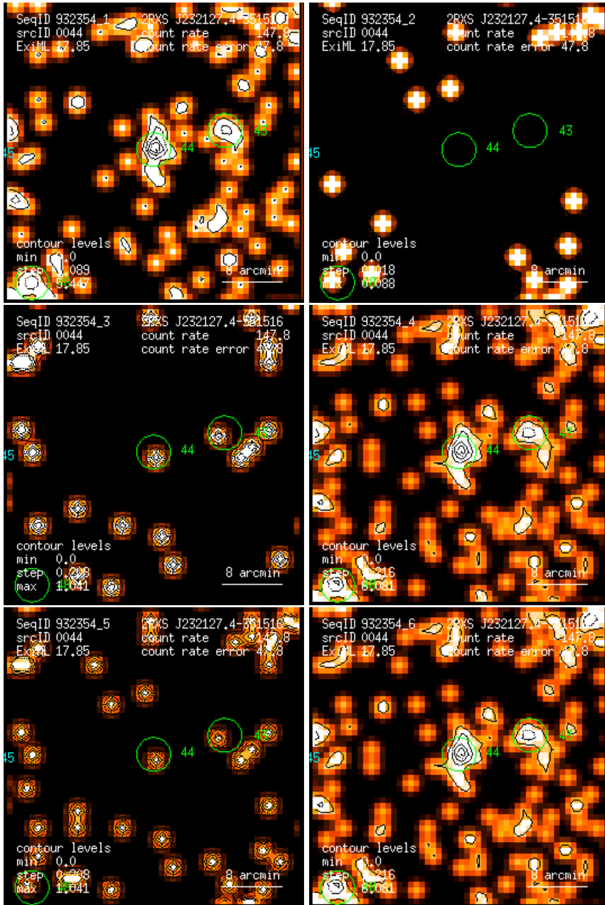
Figure 44: RASS 932354: detection 0044: band rate images, Gaussian filter: (1) PSPC channels 11 – 41, (2) 52 – 90, (3) 91 – 201, (4) 11 – 235, (5) 52 – 201, (6) 11 – 201. Broad band rates in counts/ks. Band rate contour levels in counts/ks/arcmin 2 .
