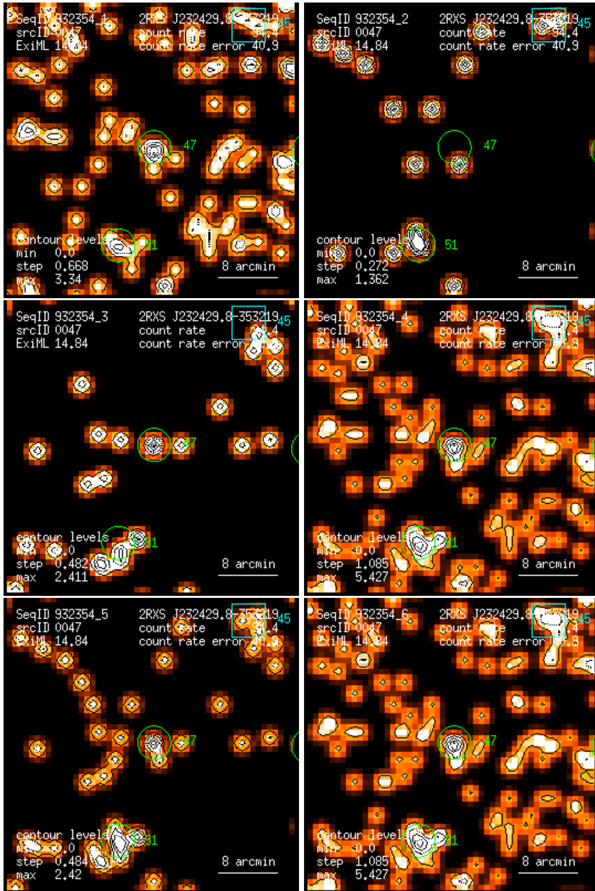
Figure 47: RASS 932354: detection 0047: band rate images, Gaussian filter: (1) PSPC channels 11 – 41, (2) 52 – 90, (3) 91 – 201, (4) 11 – 235, (5) 52 – 201, (6) 11 – 201. Broad band rates in counts/ks. Band rate contour levels in counts/ks/arcmin 2 .
