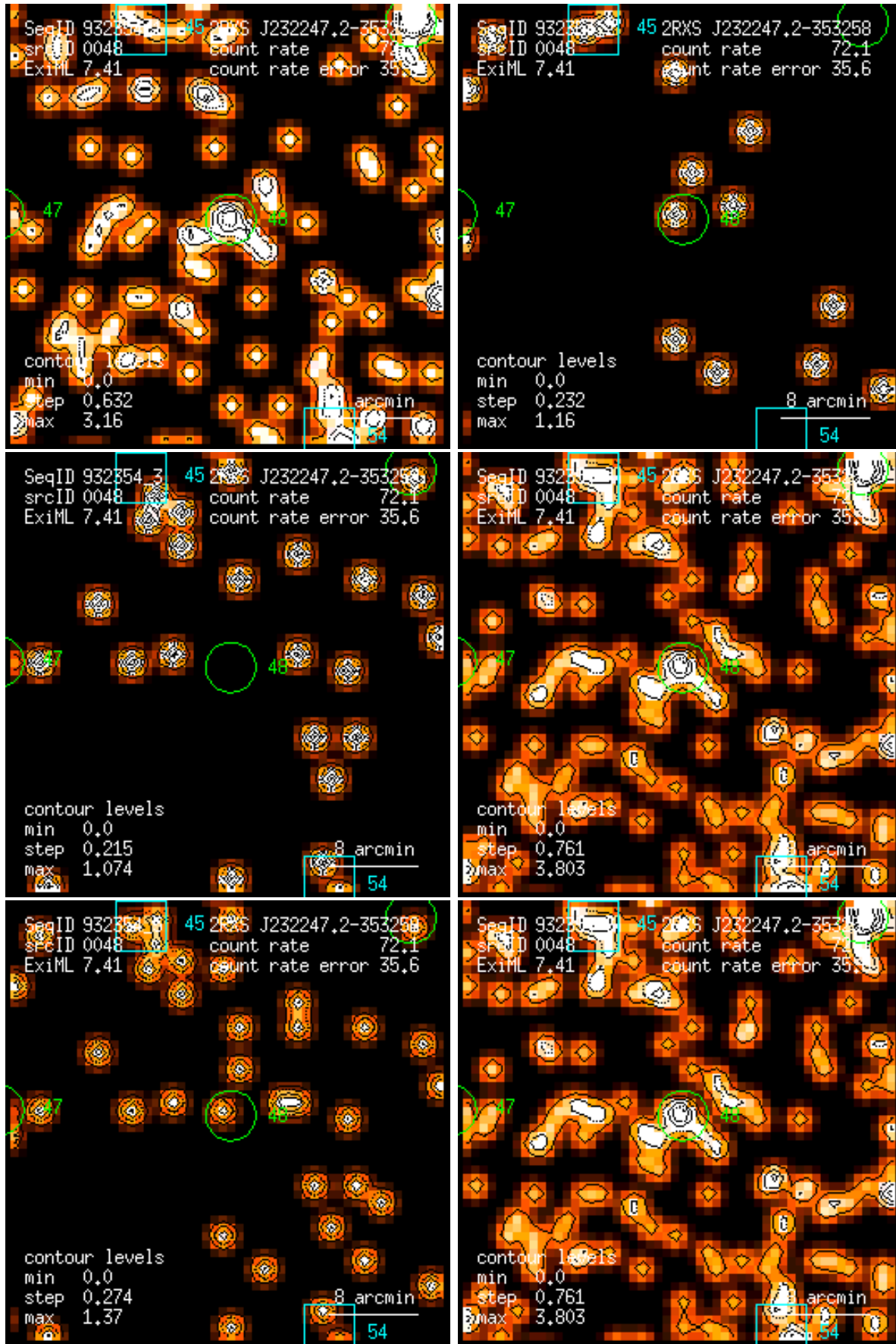
Figure 48: RASS 932354: detection 0048: band rate images, Gaussian filter: (1) PSPC channels 11 – 41, (2) 52 – 90, (3) 91 – 201, (4) 11 – 235, (5) 52 – 201, (6) 11 – 201. Broad band rates in counts/ks. Band rate contour levels in counts/ks/arcmin 2 .
