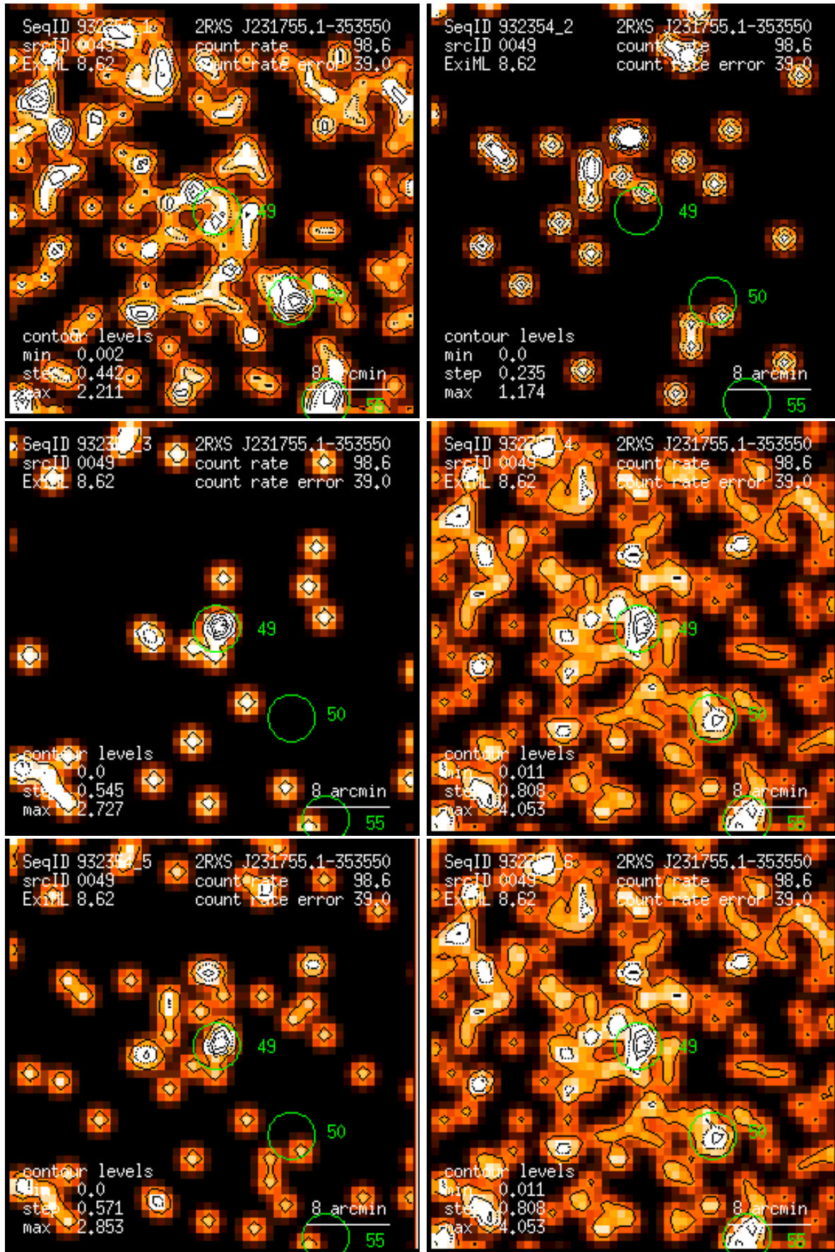
Figure 49: RASS 932354: detection 0049: band rate images, Gaussian filter: (1) PSPC channels 11 – 41, (2) 52 – 90, (3) 91 – 201, (4) 11 – 235, (5) 52 – 201, (6) 11 – 201. Broad band rates in counts/ks. Band rate contour levels in counts/ks/arcmin 2 .
